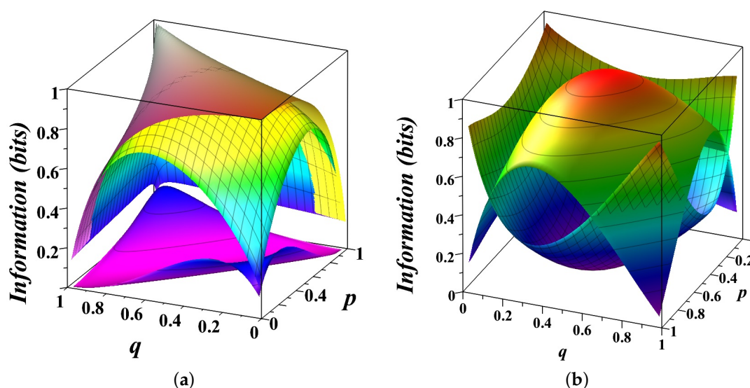
Figure 1. Decomposition of entropy H(p, q) into its components (3) for a biased coin modeled as a Markov chain T(p, q) . (a) The top surface shows the total entropy H(p, q) , the middle surface shows the entropy rate (10), and the bottom surface shows the conditional mutual information (12). The gap between the top and middle surfaces illustrates the excess entropy (9). The gap between the middle and the bottom surfaces corresponds to the unpredictable information component (14) of the system. (b) The top, convex surface shows the unpredictable component of information, reaching a maximum of 1 bit for a fair coin ( p = q = 1/2 ), but reducing to zero for a deterministic coin ( p, q = 0, 1 ). The bottom, concave surface represents the predictable component of the system, which grows as the system becomes more deterministic. Together, these surfaces illustrate the interplay between randomness and structure, showing how predictability increases as p and q deviate from 1/2 .
