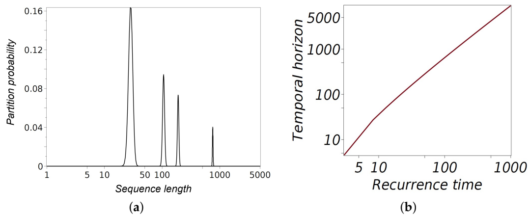
Figure 3. (a) Partition probabilities for sequences of lengths 100, 500, 1000, and 5000. The graph displays the Stirling numbers of the second kind, normalized by the corresponding Bell numbers, representing the probability of partitioning a sequence of length n into m non-empty subsets. The sharp peaks, located at m \simeq O(n/\ln n) , indicate the maxima of the Stirling numbers, highlighting the most probable partition configurations. The horizontal axis uses a logarithmic scale to effectively capture the wide range of sequence lengths. (b) Temporal horizon n as a function of recurrence time \mathcal{R} for a non-ergodic Rosencrantz coin.
