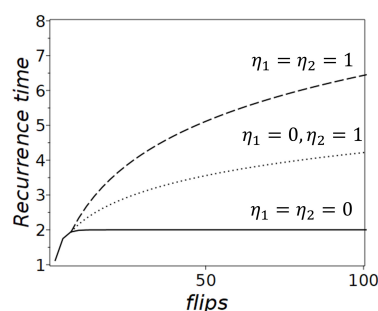
Figure 2. Recurrence times for the Rosencrantz coin model. The curves represent different \eta_1 and \eta_2 : when \eta_{1,2} = 0 (solid line), shows a stable recurrence time of 2, consistent with a fair coin and the ergodic hypothesis; \eta_1 = 0, \eta_2 = 1 (dotted line) shows gradually increasing recurrence times; when \eta_{1,2} = 1 (dashed line) shows significantly increasing recurrence times.
