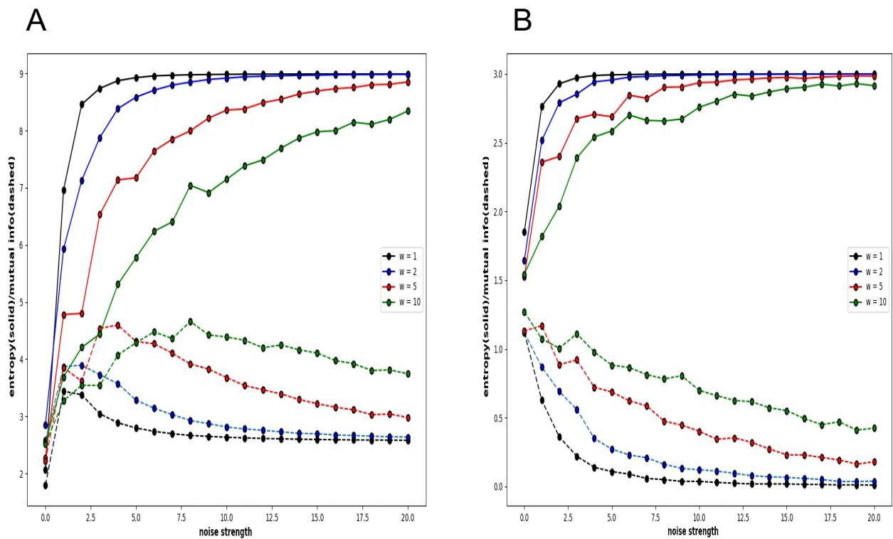
Figure 7. Four pairs of global and local entropy and mutual information plotted against noise strength for Boltzmann machine consisting of 3 \times 3 neurons under normal condition. (A). Global entropy and global mutual information. (B). Local entropy and local mutual information.
