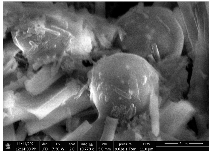
Figure 3. A scanning electron microscopy (SEM) image of uncoated proteinoid microspheres (L-Glu:L-Phe). It shows their spherical shape and distinct surface features. The image was acquired using a low field detector (LFD) at 7.50 kV accelerating voltage, with a working distance (WD) of 5.0 mm and chamber pressure of 9.82 \times 10^{-1} Torr. Imaging the non-conductive sample without a metallic coat was possible by operating under low vacuum (HFW: 11.0 \mu\text{m} ). The scale bar represents 2 \mu\text{m} at 18,778 \times magnification.
