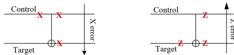
Figure 2. Schematic diagram of the error propagate of CNOT gate, where an X error propagates from the control qubit to the target qubit and a Z error propagates from the target qubit to the control qubit.
