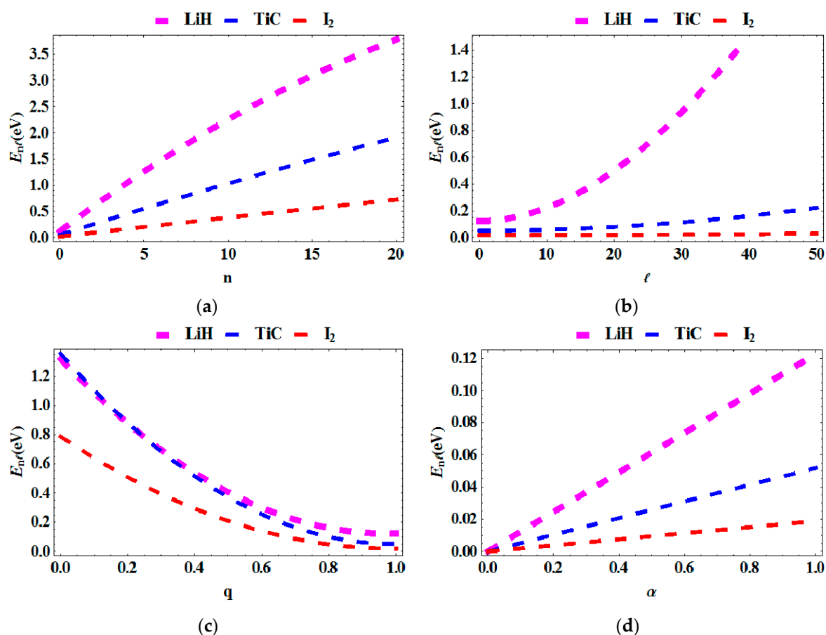
Figure 1. Energy spectra as a function of: (a) n for various diatomic molecules; (b) as a function of \ell for various diatomic molecules; (c) as a function of q for various diatomic molecules; (d) as a function of \alpha for various diatomic molecules.
