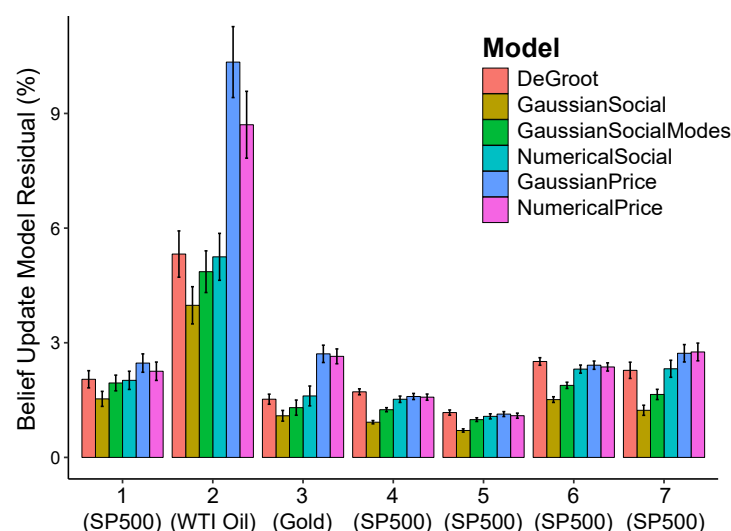
Figure 3. The y-axis shows the relative residual between modeled belief update and actual updated belief. Simple approximated models do better at modeling belief update than numerical models, and models using social histograms as likelihood perform better than models using the price history. Error bars represent 95% CI.
