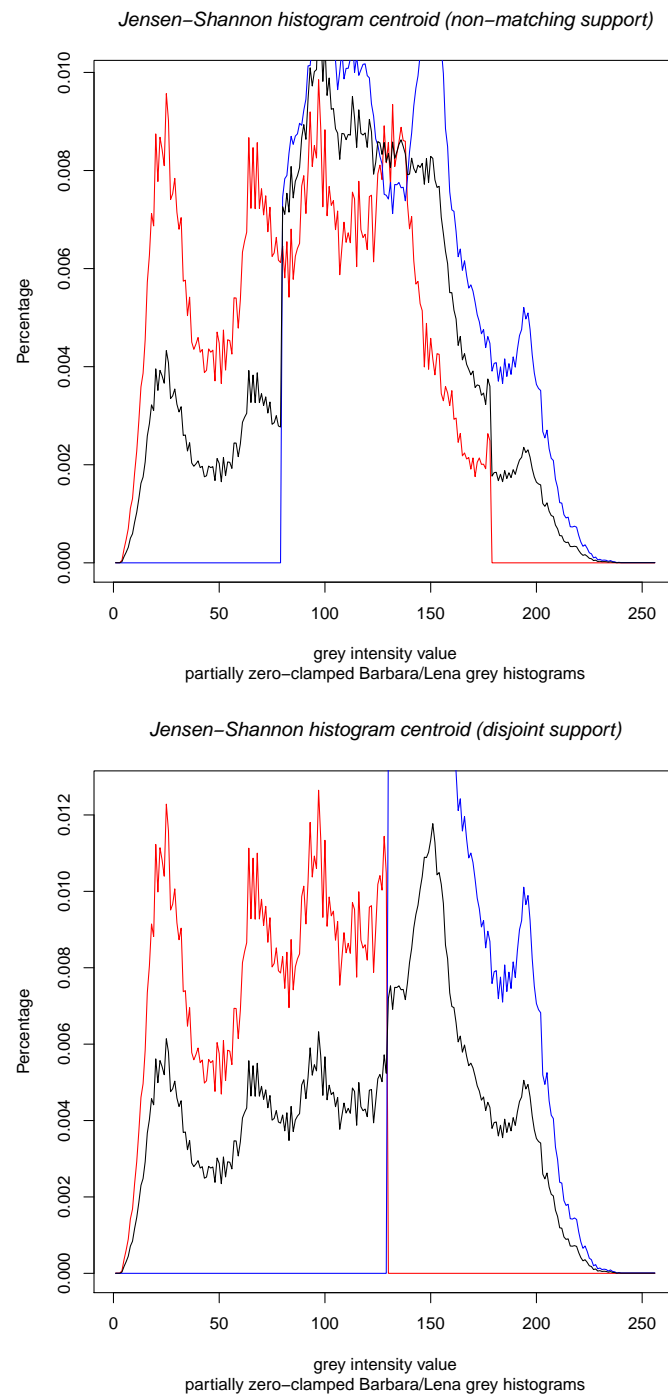
Figure 5. Jensen–Shannon centroid (black histogram) for the clamped grey normalized histogram of the Lena image (red histograms) and the clamped gray normalized histogram of Barbara image (blue histograms). Notice that on the part of the sample space where only one distribution is non-zero, the JS centroid scales that histogram portion.
