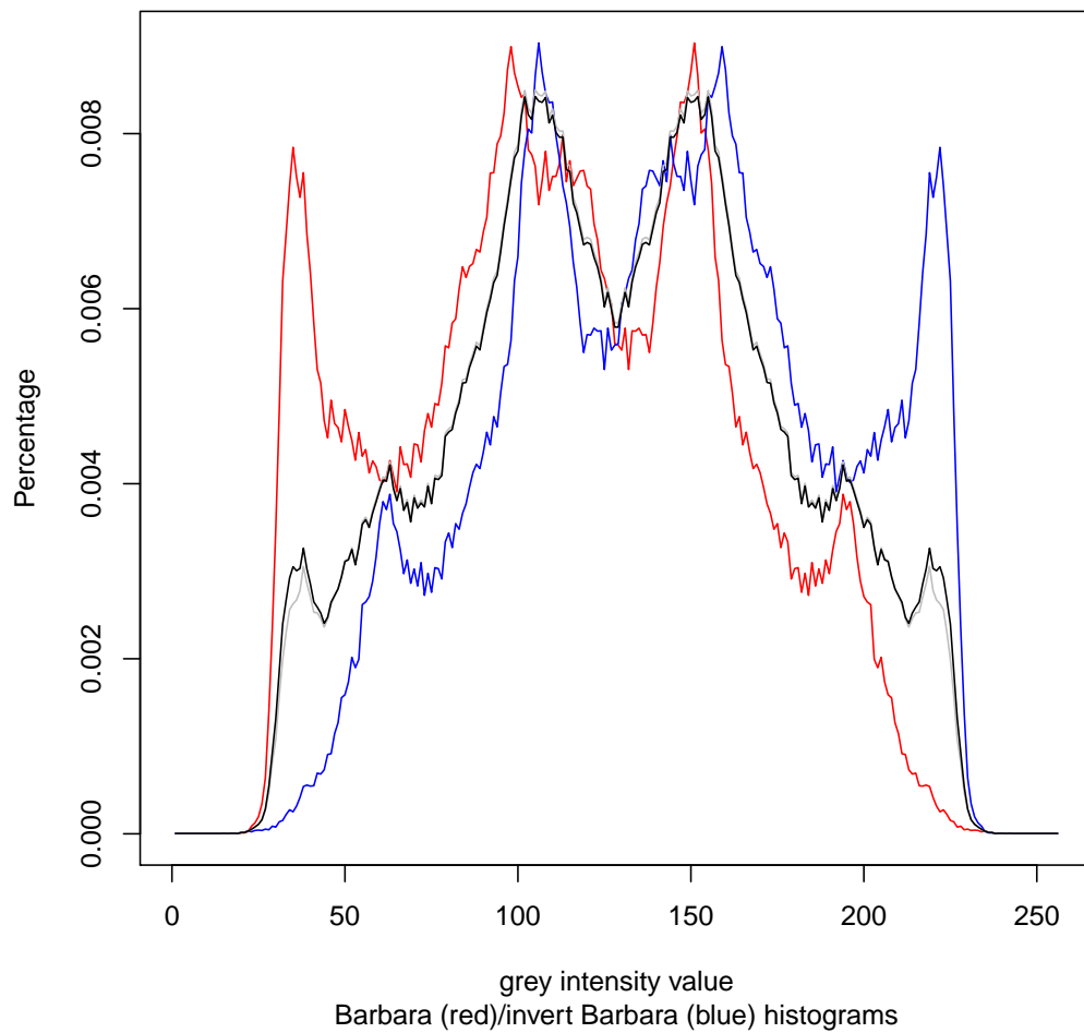
Figure 4. The Jeffreys centroid (grey histogram) and the Jensen–Shannon centroid (black histogram) for the grey normalized histogram of the Barbara image (red histogram) and its negative image (blue histogram which corresponds to the reflection around the vertical axis x = 128 of the red histogram).
