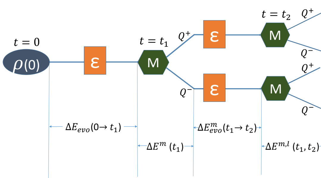
Figure 1. Schematic diagram for the energy change \Delta E_{1,2}^{m,l} . Here, we take a general dichotomic measurements Q^\pm as an example with m, l = \pm 1 being the measurement outcomes, and \varepsilon is the system propagator \rho \rightarrow \varepsilon(\rho) .
