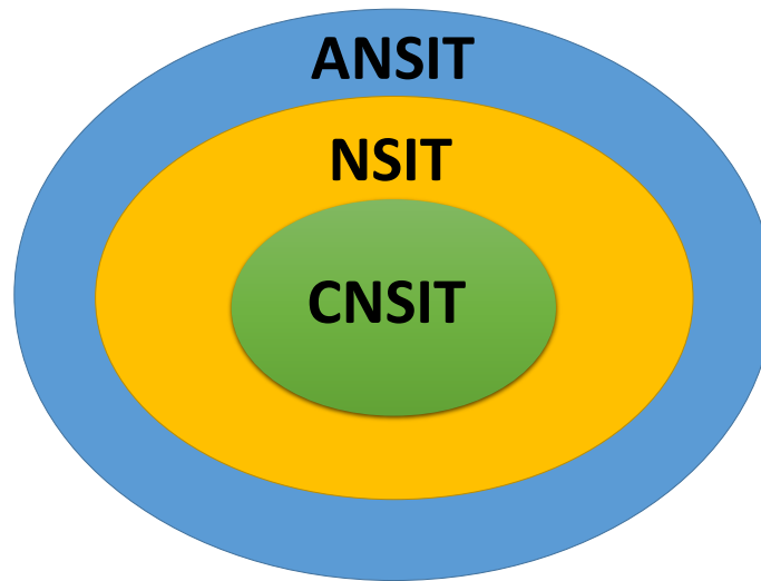
Figure 3. Schematic diagram for the relationship among the NSIT conditions, the CNSIT conditions and the ANSIT conditions in the case of the driven qubit and the dissipative qubit, respectively.
