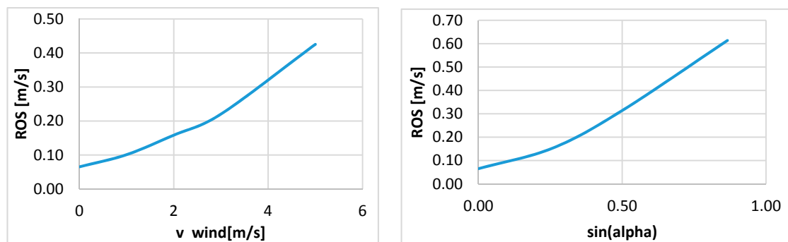
Figure 4. WFDS simulation results for different slope and wind speed.
