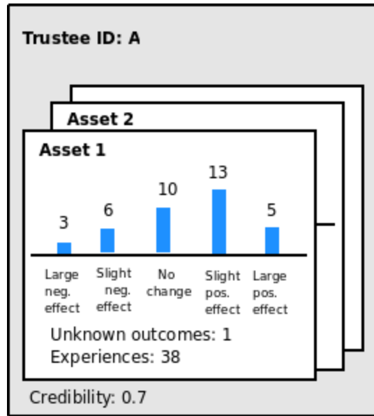
Figure 4: A Sample External Reputation View.
