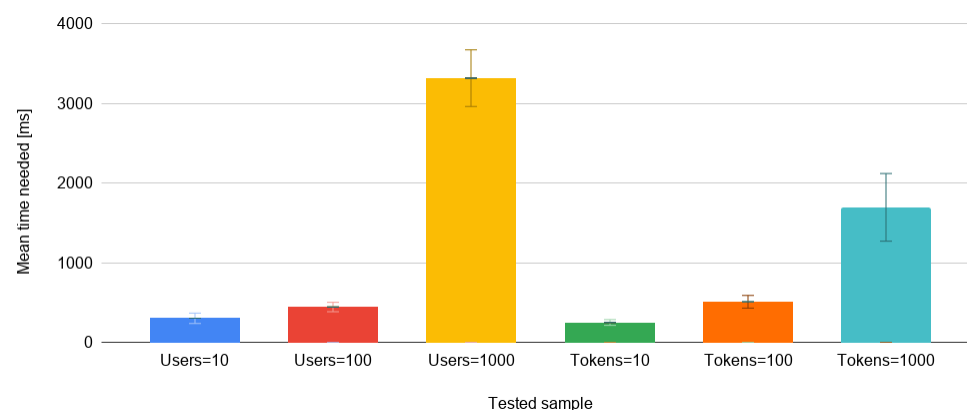
Figure 4. User and token registration transfer times.
