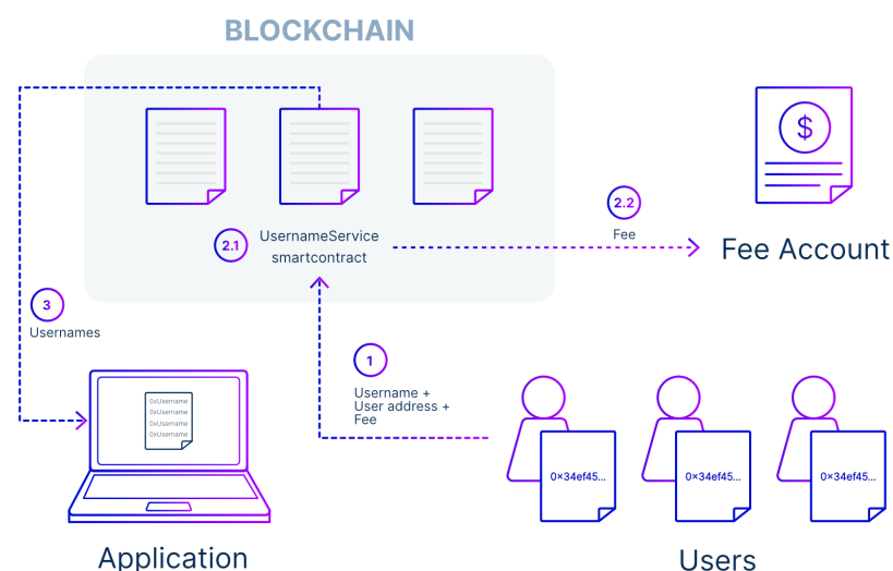
Figure 2. Workflow of Account Aliasing System.
