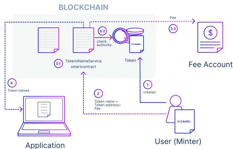
Figure 3. Workflow of Tokens Name Service.
