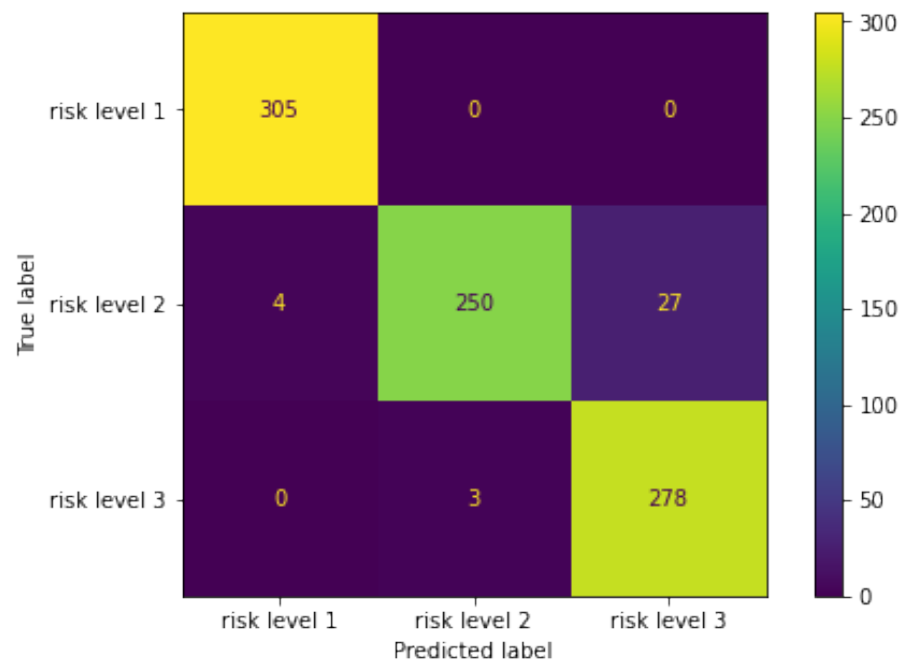
Figure 8. Confusion matrix of route risk level prediction model. The matrix shows the three classes of route risk level (1 for low risk, 2 for medium risk, and 3 for high risk).
