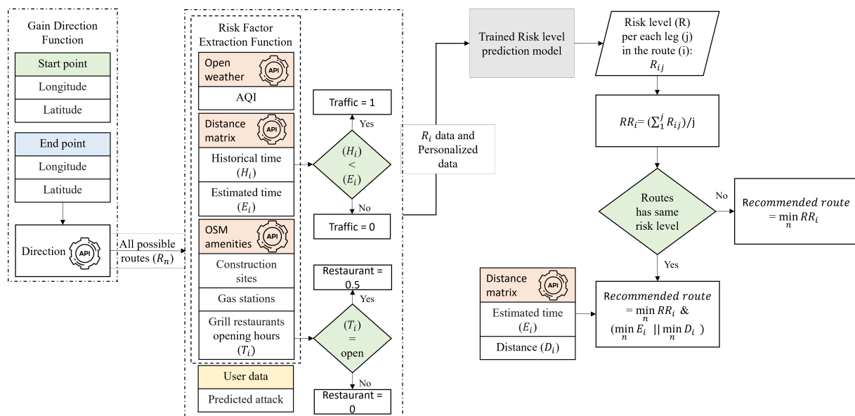
Figure 2. Flowchart of the proposed safe route recommendation model showing the gain direction and risk factor extraction functions.
