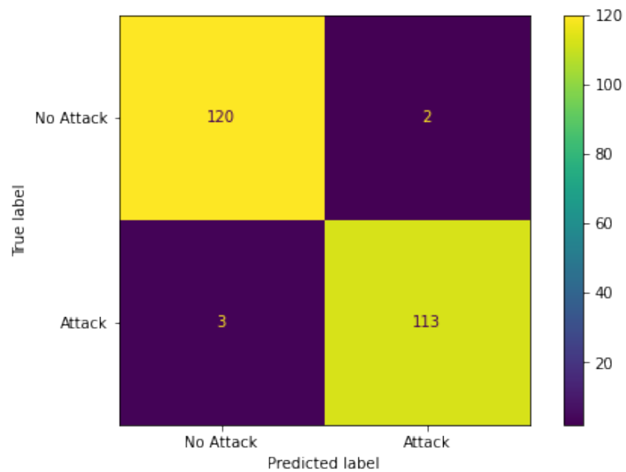
Figure 7. Confusion matrix of asthma attack prediction model. The matrix shows the two classes of asthma attack prediction (Attack and No Attack).
