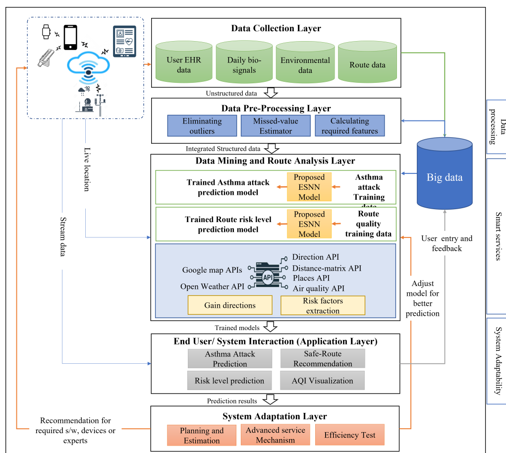
Figure 1. Proposed framework of the smart eHealth system. The framework shows the system layers with the flow of input and output between these layers.
