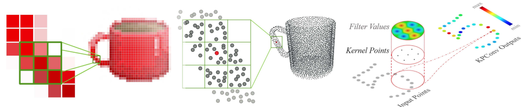
Figure 16. Left: pixel-wise convolution with kernel size 3 \times 3 . Center: Pointwise convolutions: For each point, nearest neighbors are searched and binned into kernel cells before convolving with kernel weights. Graphic originally shown in [138]. Right: Kernel point convolution 2D example. Input points with a constant scalar feature (in grey) are convolved through a KPConv that is defined by a set of kernel points (in black) with filter weights on each point. The graphic was originally shown in [100].
