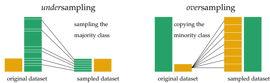
Figure 8. Graphical representation of the two principles of under- and oversampling for imbalanced training data handling in machine learning applications.
