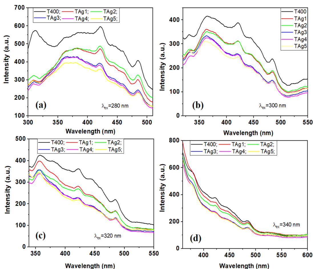
Figure 7. Emission spectra of pure \text{TiO}_2 and Ag– \text{TiO}_2 nanostructured nanofibers at different excitation wavelengths \lambda_{\text{ex}} = 280 nm (a), 300 nm (b), 320 nm (c) and 340 nm (d).
