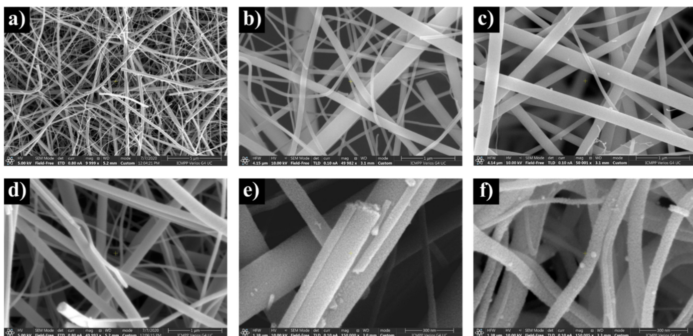
Figure 2. Small and larger magnification SEM images of Ag–TiO 2 nanostructured nanofibers: pure TiO 2 \times 10,000 (a), 0.1% Ag–TiO 2 \times 50,000 (b), 5.0% Ag–TiO 2 \times 50,000 (c), TiO 2 \times 50,000 (d), 0.1% Ag–TiO 2 \times 150,000 (e), and 5.0% Ag–TiO 2 \times 150,000 (f).
