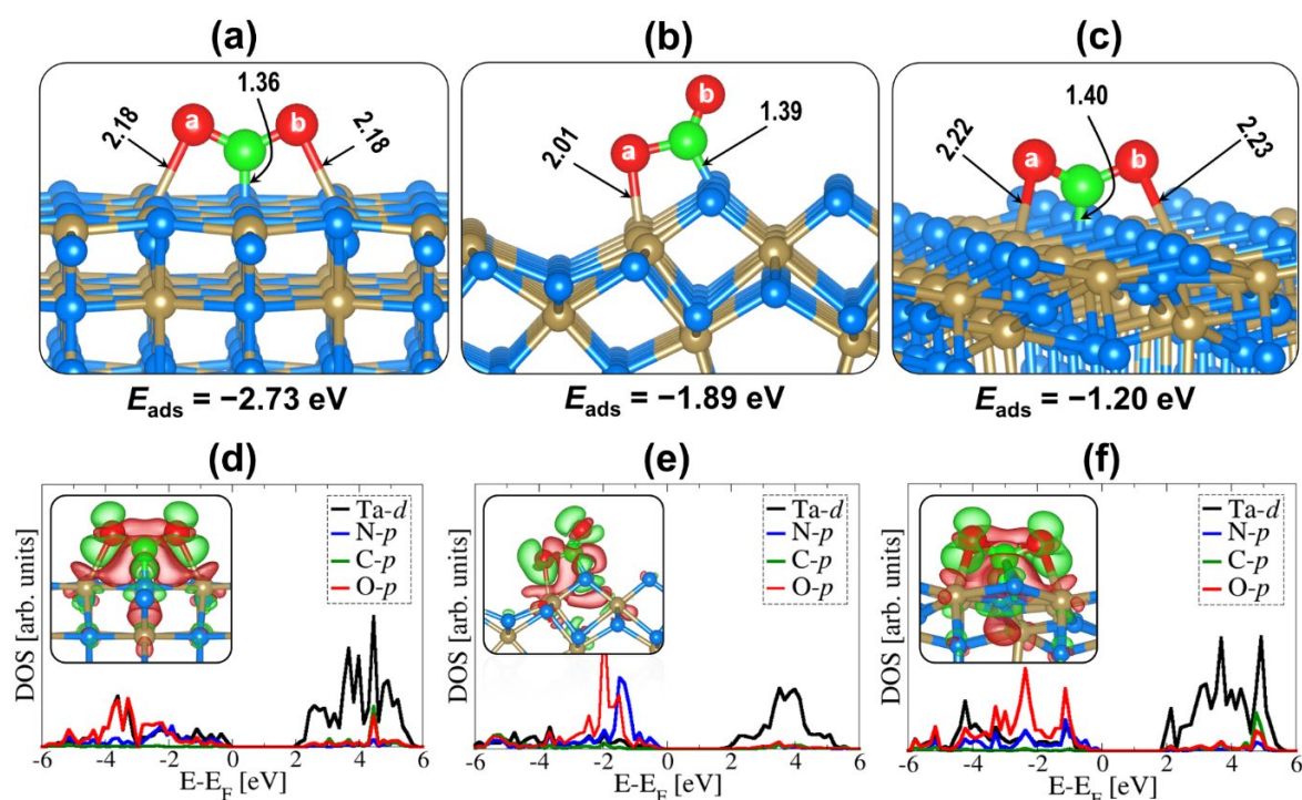
Figure 4. Lowest-energy \text{CO}_2 adsorption structures on (a) (001), (b) (010), and (c) (110) \text{Ta}_3\text{N}_5 surfaces. The DOS projected on the surface Ta d states and N p states interacting with the C and O p states of \text{CO}_2 (d–f) and the corresponding isosurface contours of the differential charge density are shown as inserts in (d–f), where green contours denote electron density increase and the red contours denote electron density decrease by 0.02 \text{ e}/\text{\AA}^3 , respectively. (Atomic colour scheme: Ta = pale olive, N = blue, C = green, and O = red.)
