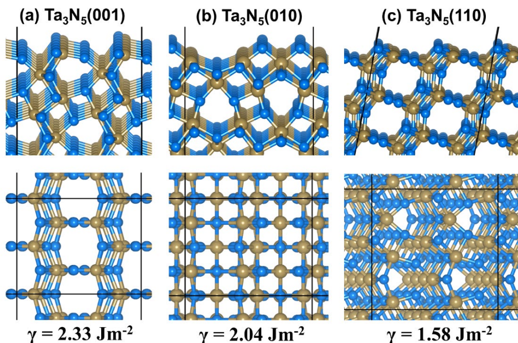
Figure 2. Optimized structures of the (a) \{001\} – (2 \times 1) , (b) \{010\} – (2 \times 1) , and (c) \{110\} – (1 \times 1) surfaces of \text{Ta}_3\text{N}_5 , in top (top) and side (bottom) views. (Atomic colour scheme: Ta = pale olive and N = blue.)
