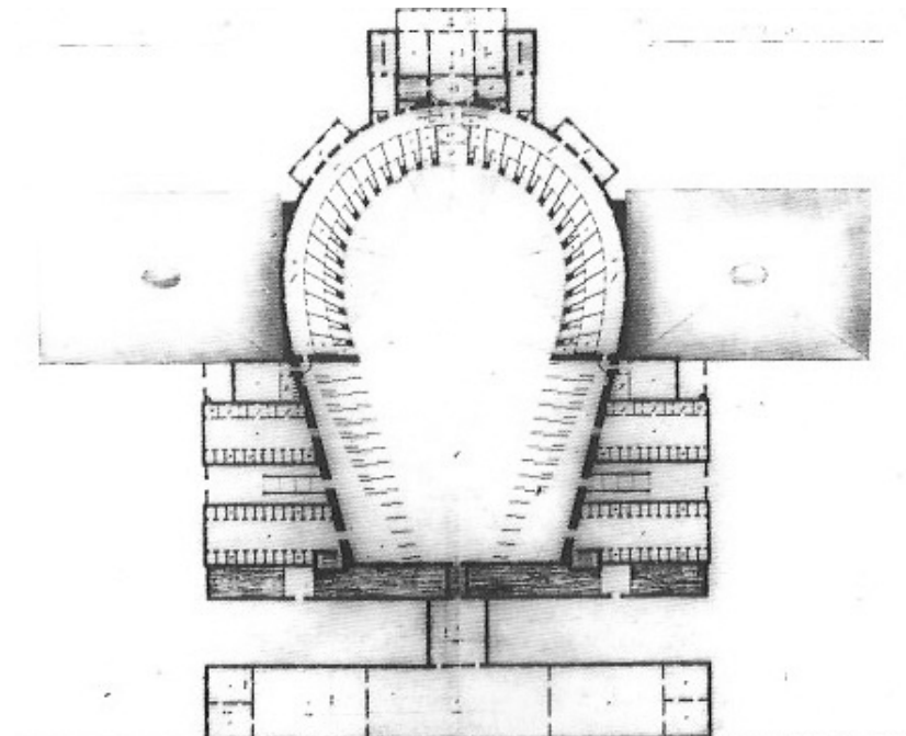
Figure 14. Ideal theatre shape according to Tommaso Carlo Beccega (1817) (after [83]).
