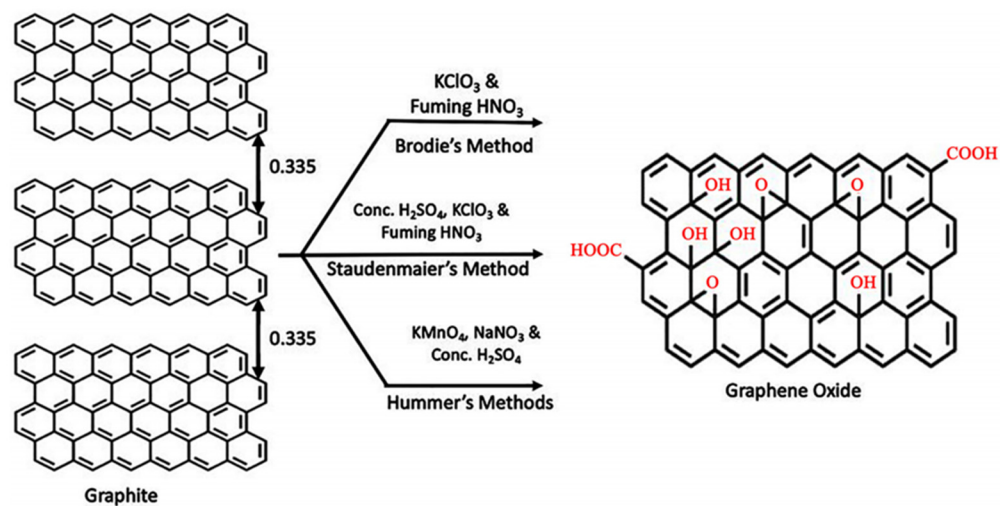
Figure 11. Fabrication techniques of Graphene oxide [121].
