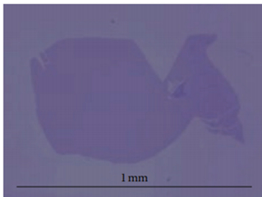
Figure 12. Single layered graphene synthesised by mechanical exfoliation on Si/SiO 2 [102].
