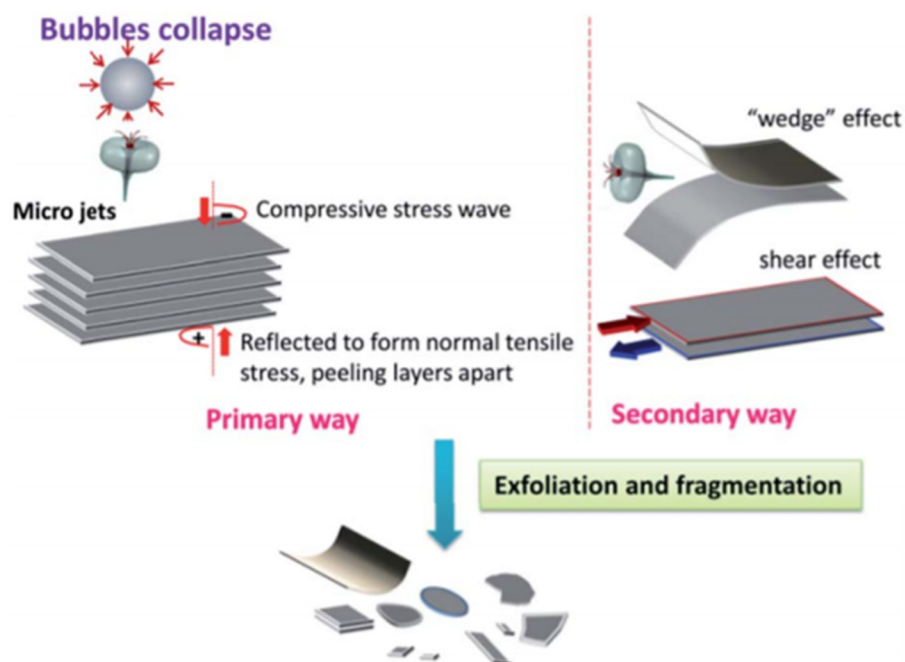
Figure 10. Schematic figure of mechanical exfoliation of graphene by sonication method. “Reproduced with permission from [111], [Journal of Materials Chemistry A]; published by [Royal Society of Chemistry], 2015”.
