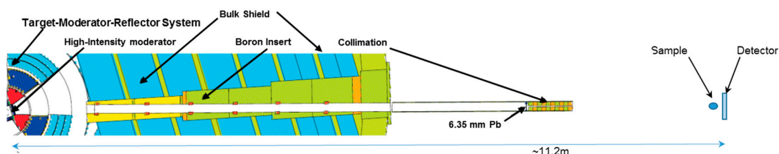
Figure 4. Flight Path 05 Schematic. Beyond the first 10 m station, there is an evacuated pipe and some large diameter polyethylene shielding leading to the 60 m station.
