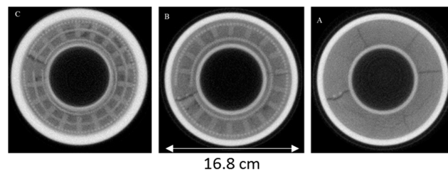
Figure 16. High-energy neutron CT scan of a heavy tungsten-encased ceramic cathode assembly—cathode is shown in front of flat panel in Figure 15 left photo. Cracks in the ceramic are difficult to impossible to image with X-rays. Slices in three different planes show (A) ceramic with cracks (B) spiral wound heating element near edge and center of ceramic (C) central support of heating element.
