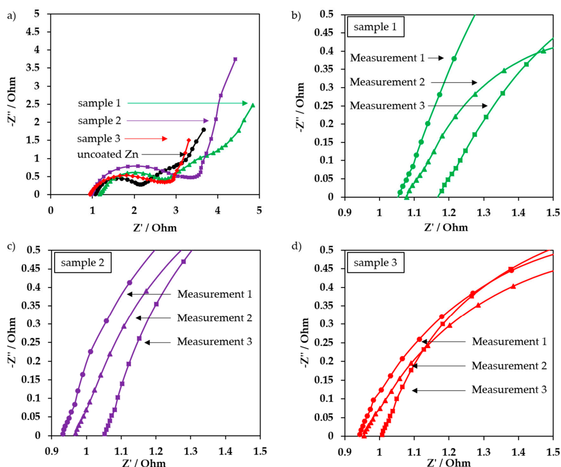
Figure S1. (a) Exemplary Nyquist plots of uncoated zinc, sample 1, sample 2 and sample 3. (b–d) Zoom on high-frequency region of EIS to determine R_i from three measurements for sample 1, sample 2, and sample 3
