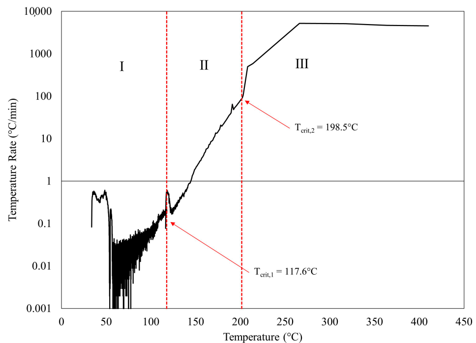
Figure 1. Determination of temperature rate (TR) critical temperatures [6].
