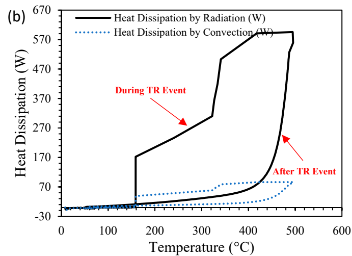
Figure 8. (a) Samsung 30Q 18650 heat dissipation during the TR event. (b) 20 Ah pouch cell heat dissipation during the TR event.
