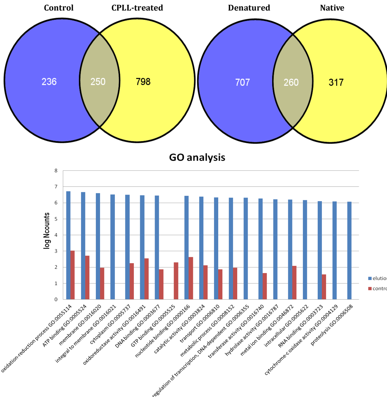
Figure 2. Upper panel: Venn diagrams showing the total identifications of avocado proteins in either the control or in the CPLL treated samples (left diagrams). The Venn diagrams to the right display the relative contributions to the total IDs of the denatured vs. the native sample extractions. Lower panel: GO analysis of the proteins detected in various metabolic processes in the control vs. CPLL-treated samples. In the latter case, five additional metabolic processes can be described, which are not visible in the control sample and most likely represent low- to very-low abundance proteins, whose visibility has been substantially enhanced via the CPLL technology (modified from Esteve et al. [43]).
