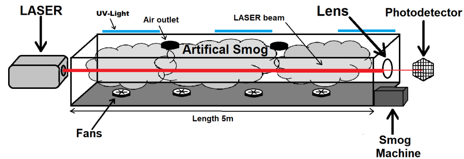
Figure 1. Block diagram.
