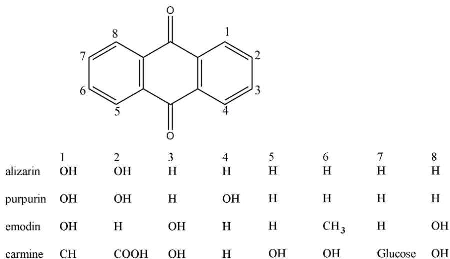
Figure 1. (a) The structure of anthraquinones and the position of the substituted group. (b) The structure of flavones, flavonols and the position of the substituted group.
