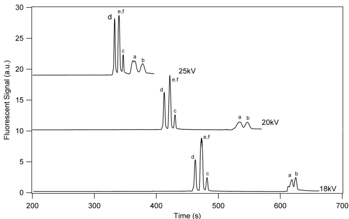
Figure 4. Separation of selected flavonoid dyes (a) 0.5 \mu\text{g mL}^{-1} kaempferol, (b) 2 \mu\text{g mL}^{-1} luteolin, (c) 1 \mu\text{g mL}^{-1} apigenin (d) 2 \mu\text{g mL}^{-1} myricetin, (e) 1 \mu\text{g mL}^{-1} quercetin, (f) 0.5 \mu\text{g mL}^{-1} morin, in 20 mM borate buffer (pH = 8.0) and 20 mM SDS with 5% acetonitrile and an applied potential of 18, 20 and 25 kV.
