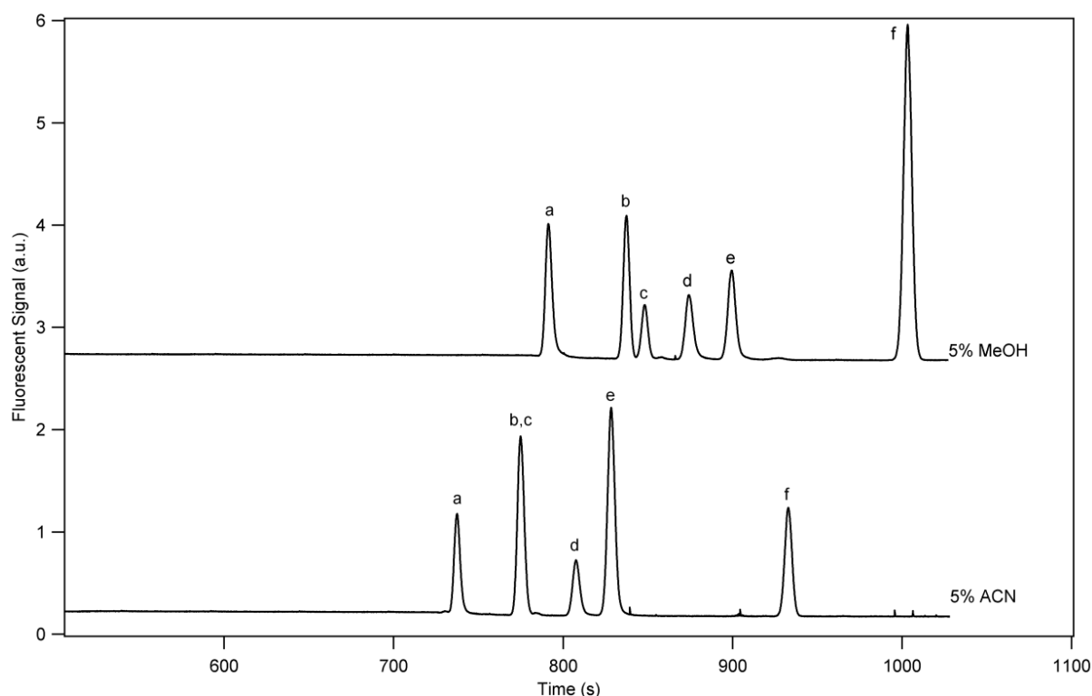
Figure 2. Separation of the flavonoid dyes: (a) 0.5 \mu\text{g mL}^{-1} kaempferol, (b) 1 \mu\text{g mL}^{-1} luteolin (c) 2 \mu\text{g mL}^{-1} apigenin, (d) 2 \mu\text{g mL}^{-1} myricetin, (e) 1 \mu\text{g mL}^{-1} quercetin, (f) 0.5 \mu\text{g mL}^{-1} morin, in 5% (v/v) of acetonitrile or 5% (v/v) methanol, at 18 kV, 20 mM borate buffer (pH = 9.24) and 20 mM sodium dodecyl sulfate (SDS).
