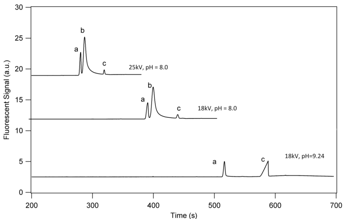
Figure 5. Separation of selected anthraquinones (a) 10 \mu\text{g mL}^{-1} alizarin, (b) 3 \mu\text{g mL}^{-1} purpurin, (c) 10 \mu\text{g mL}^{-1} emodin in 20 mM borate buffer (pH = 9.24 and 8.0) and 20 mM SDS, using an applied potential of 18 and 25 kV.
