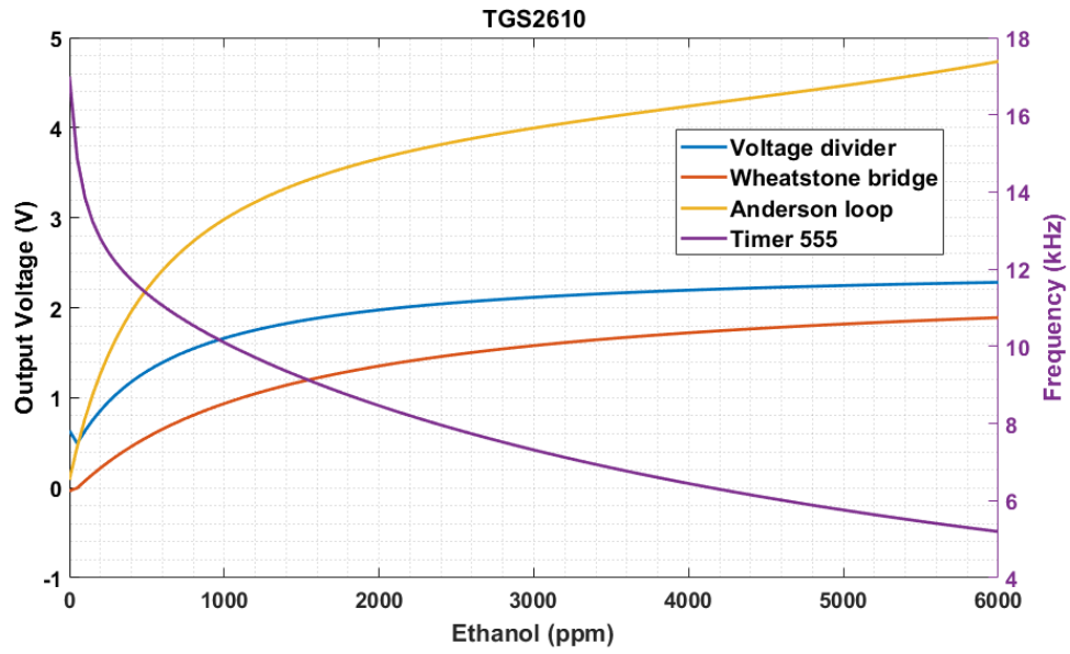
Figure S7. Output models for each topology using the TGS2600 sensor.
