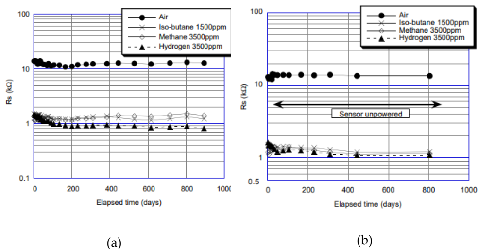
Figure S2. (a) Long-term stability of sensor TGS2610 when the sensor is continuous energizing [16]. (b) Long-term stability of sensor TGS2610 when the sensor is unenergized between measures [16].
