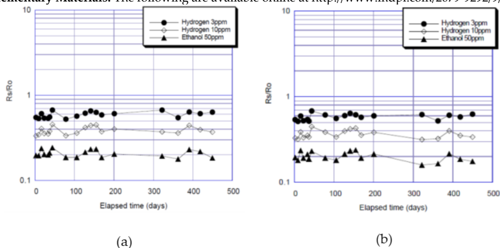
Figure S1. (a) Long-term stability of sensor TGS2600 when the sensor is continuous energizing [15]. (b) Long-term stability of sensor TGS2600 when the sensor is unenergized between measures [15].
