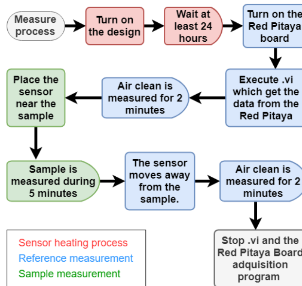
Figure S5. Measurement process steps.
