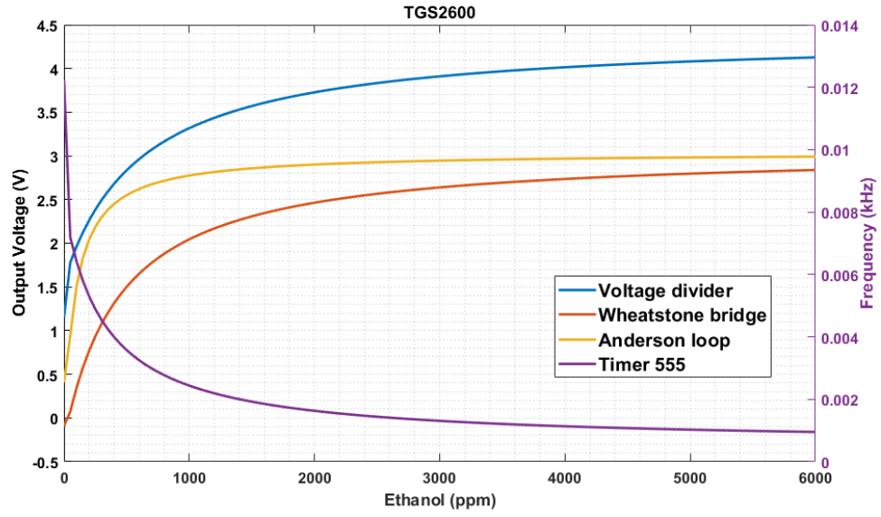
Figure S6. Output models for each topology using the TGS2600 sensor.
