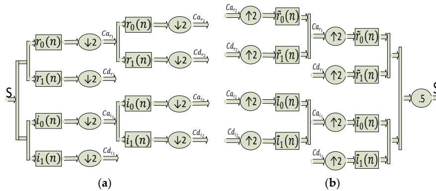
Figure 1. The two-level filter bank implementation of (a) DTCWT and (b) IDTCWT.
