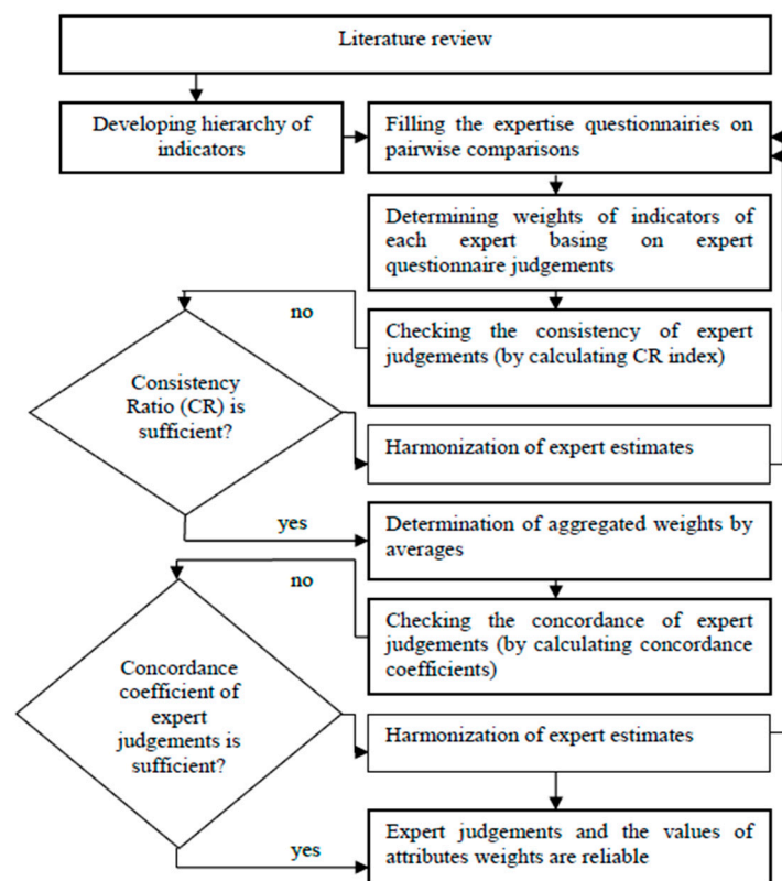
Figure 1. Research methodology.
