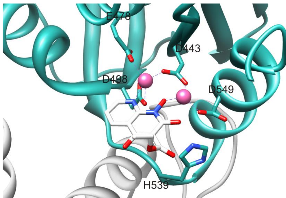
Figure 6. Binding of the N-hydroxy naphthyridinone inhibitor MK1 to the RT RNase H active site. The figure is derived from PDB file 3LP0 and was drawn using UCSF Chimera software [6]. Dashed lines indicate interactions with the metal cations.
