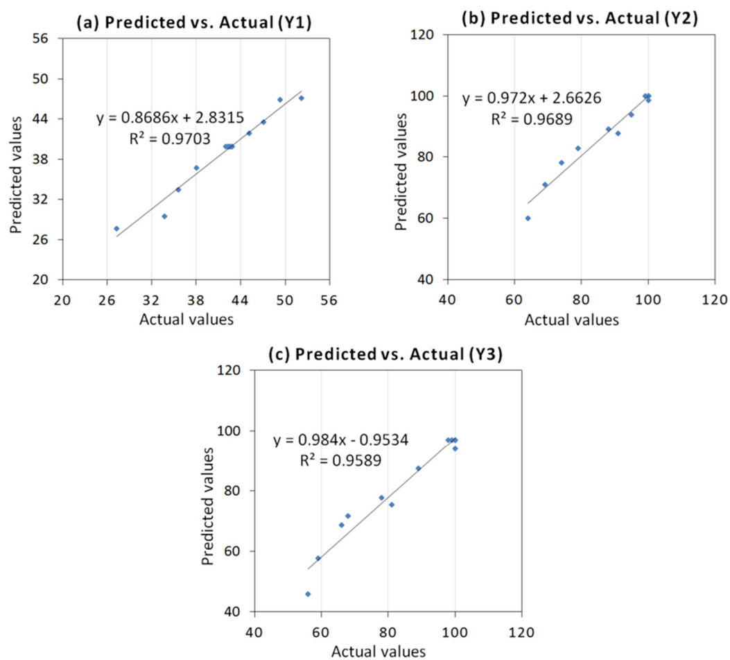
Figure I. Predicted vs experimental values for (a) UV protection factor (UPF), (b) %reduction of E.coli , and (c) %reduction of S.aureus
