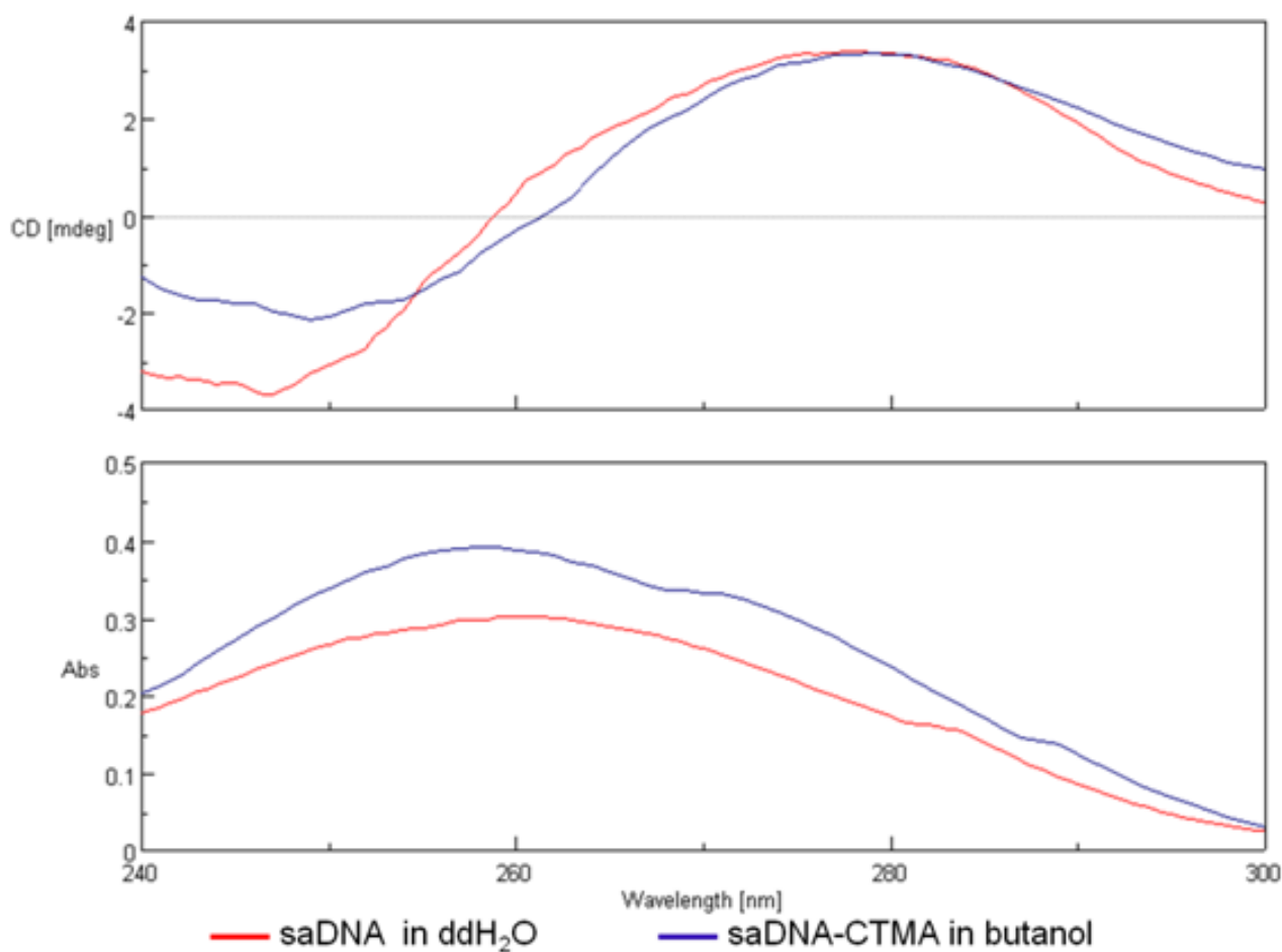
Figure S1. CD spectroscopy of SaDNA (red) in aqueous solution and saDNA-CTMA (blue) in butanol.
