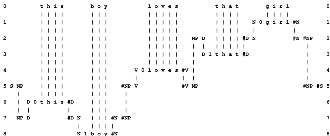
Figure 4. The best multiple alignment found by the SP model with the New pattern “t h i s b o y l o v e s t h a t g i r l” and a set of user-supplied Old patterns representing some of the grammatical forms of English, including words with their grammatical markers.
