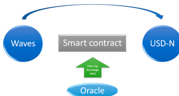
Figure 2. Crypto swap including an oracle.
