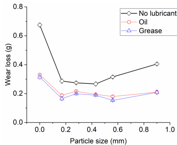
Figure 7. Average wear loss of straw powder with different particle sizes under various lubrication conditions.
