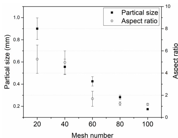
Figure 1. Particle size and aspect ratios of straw powder after screening with different mesh numbers.
