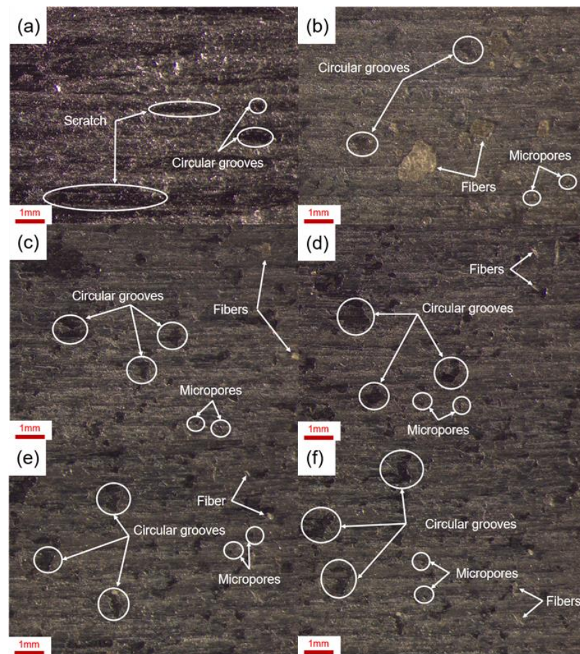
Figure 9. Worn disk surfaces with various particle sizes under lubricating oil condition: (a) no powder added; (b) 0.17 mm; (c) 0.28 mm; (d) 0.43 mm; (e) 0.56 mm; (f) 0.90 mm.
