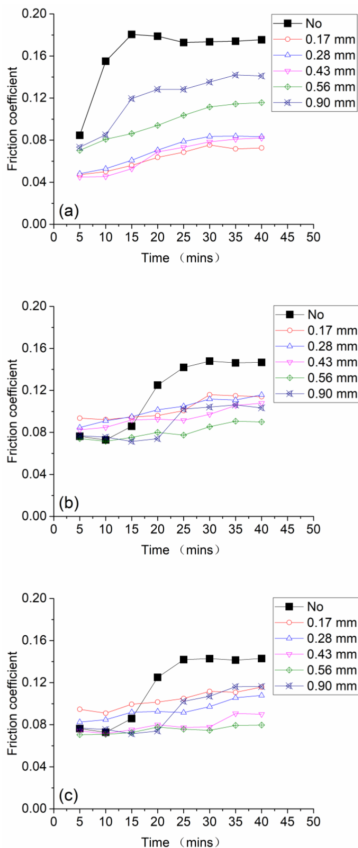
Figure 3. Variation curves of friction coefficient between steel–straw powder–steel with different particle sizes: (a) no lubricant; (b) lubricating oil; (c) lubricating grease.
