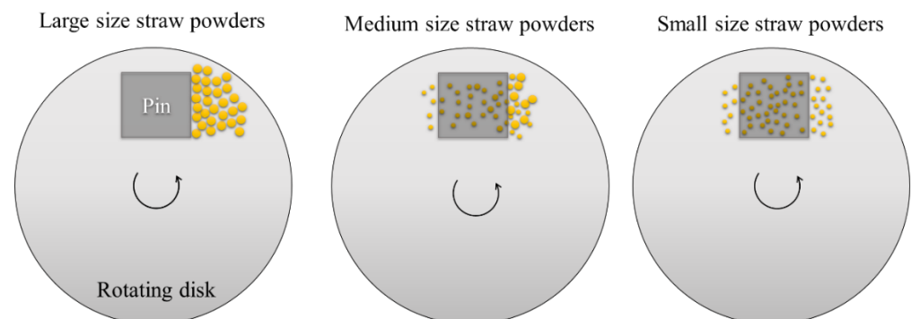
Figure 5. Movement of straw powder with different particle sizes during friction.
