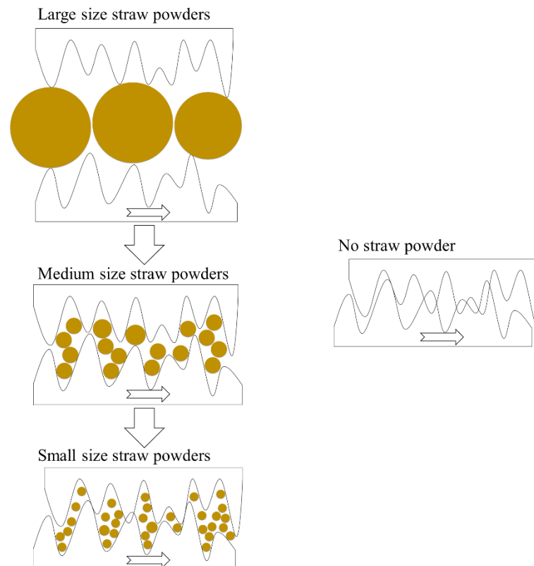
Figure 6. Behavior and evolution process of straw powders with different particle sizes at the contact interface.
