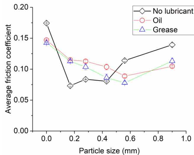
Figure 4. Average friction coefficient of straw powder with different particle sizes under various lubrication conditions.
