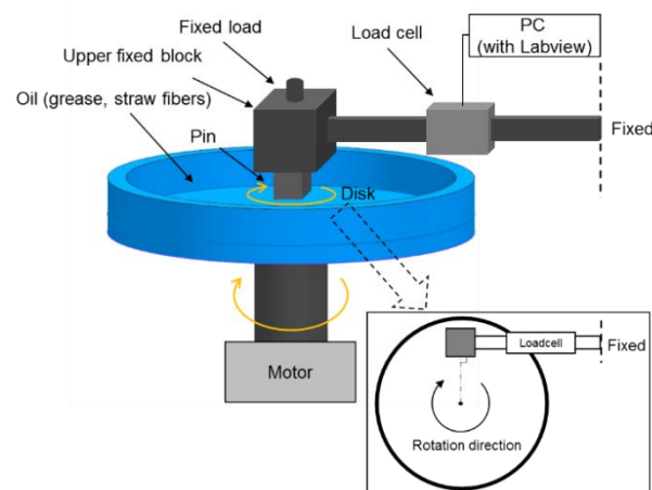
Figure 2. Pin-on-disk friction and wear tester.
