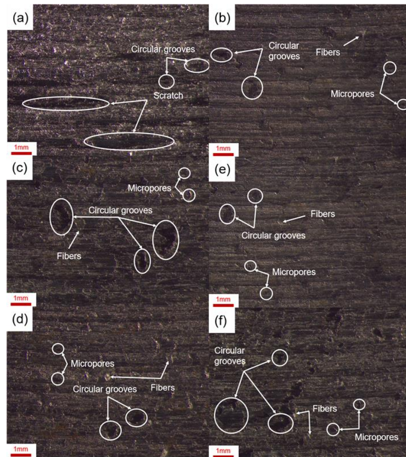
Figure 10. Worn disk surfaces with various particle sizes under lubricating grease condition: (a) no powder added; (b) 0.17 mm; (c) 0.28 mm; (d) 0.43 mm; (e) 0.56 mm; (f) 0.90 mm.
