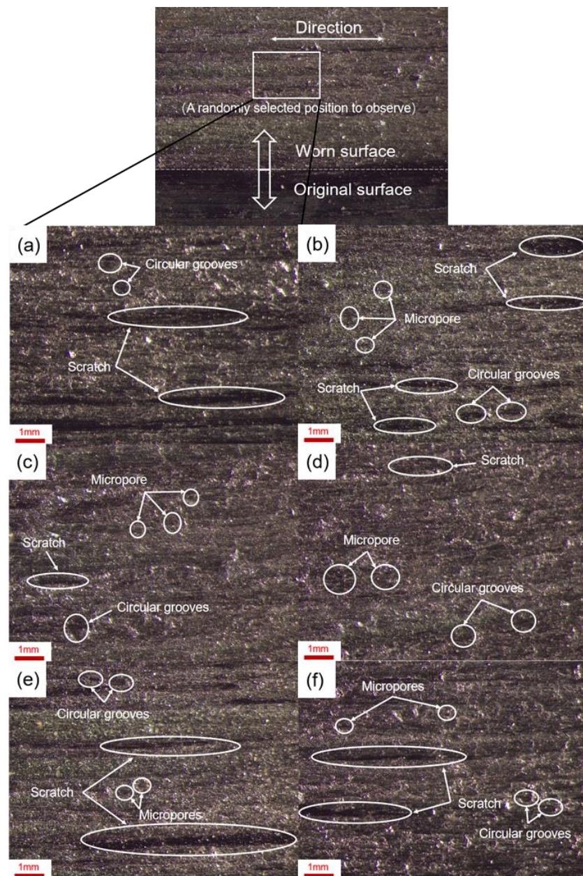
Figure 8. Worn disk surfaces with various particle sizes under no lubricant condition: (a) no powder added; (b) 0.17 mm; (c) 0.28 mm; (d) 0.43 mm; (e) 0.56 mm; (f) 0.90 mm.
