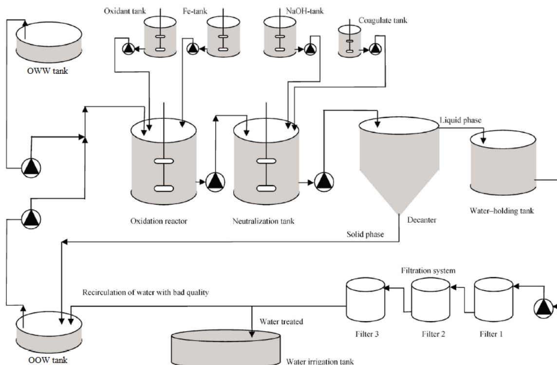
Figure 3. Scheme of the industrial treatment plant for OMW-2 located in Jaén (Spain).
