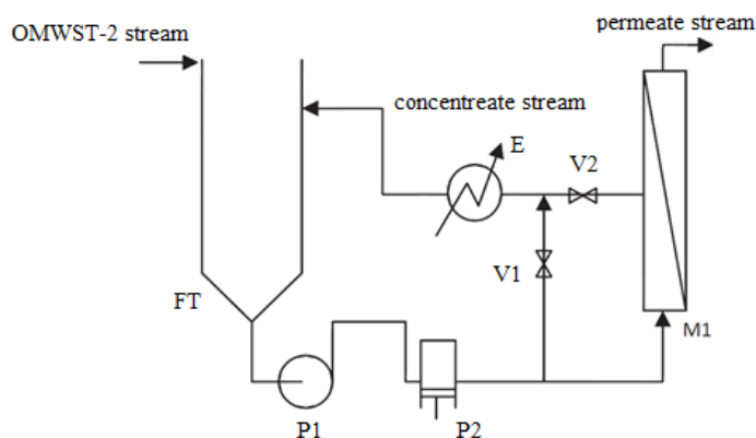
Figure 4. Membrane filtration pilot plant flow scheme. FT: feed tank; P 1 : booster pump; P 2 : volumetric pump; V 1 : bypass regulation valve; V 2 : concentrate regulation valve; E: plate heat exchanger; M 1 : membrane housing provided with SW membrane.
