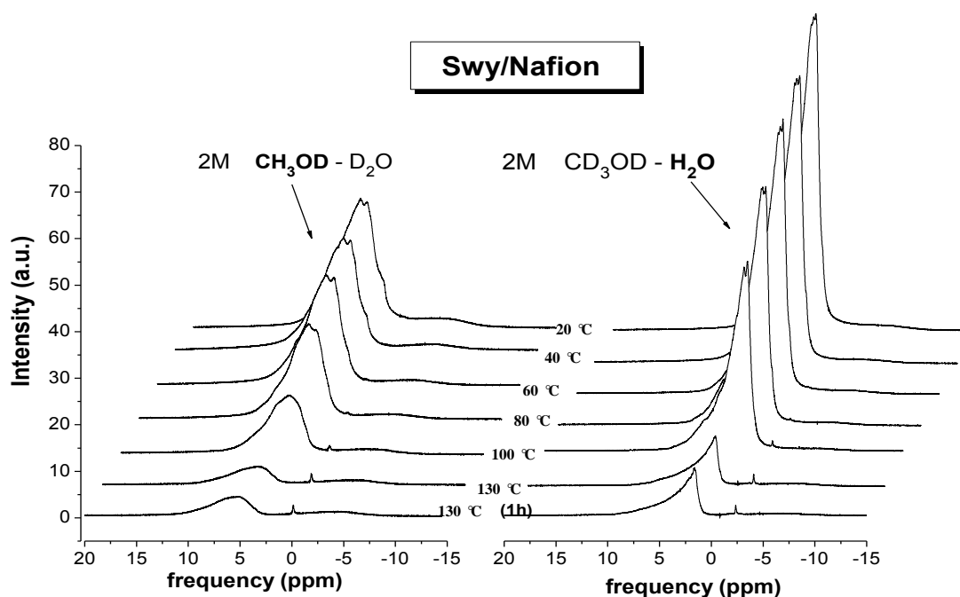
Figure 5. Evolution of proton spectra from methanol (on the left) and water (on the right) as a function of temperature on Swy/Nafion composite swollen in 2 M methanol solution. The spectra were referenced setting methyl protons and pure water at 0 ppm, respectively.
