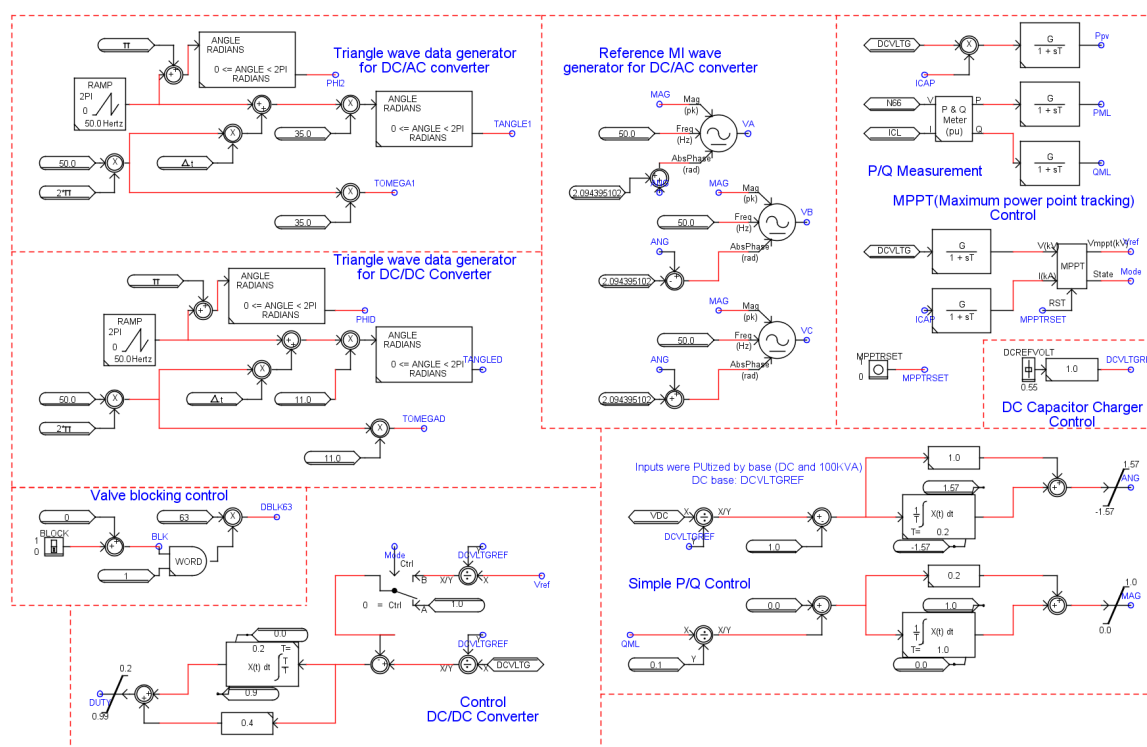
Figure S1. Block diagram implementation of the single phase PV control system developed in RSCAD.
