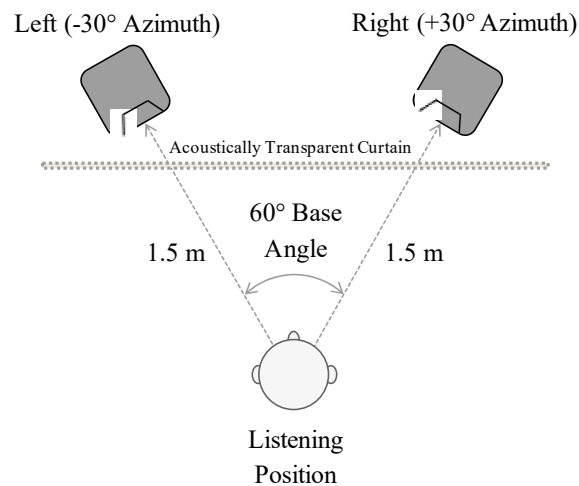
Figure 4. Horizontal loudspeaker setup with a 60° base angle.
