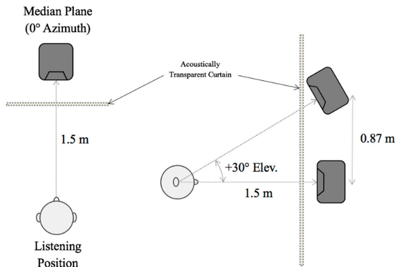
Figure 5. Vertical loudspeaker setup at 0° azimuth with a +30° elevation.
