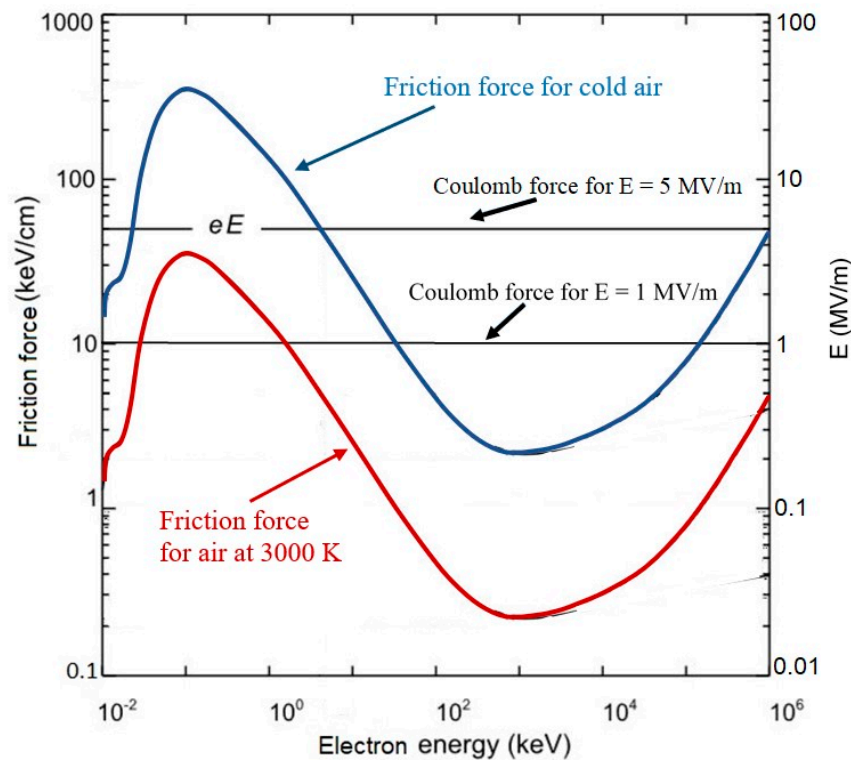
Figure 1. The dynamic friction curves showing the friction force (rate of energy loss per unit distance) experienced by an electron as a function of electron energy for cold air and for air at 3000 K. The curves include the effects of both inelastic scattering of the electron with air molecules and Bremsstrahlung emission. The horizontal lines represent the Coulomb force acting on the electron ( eE , where E is the electric field intensity and e is the electron charge) corresponding to E = 1 MV/m and E = 5 MV/m (see the right vertical scale). Electrons can run away to relativistic energies when the Coulomb force is greater than the friction force. For cold air and E = 5 MV/m, only electrons with energy greater than 5 keV can run away, while for the air at 3000 K, all electrons can do so. Adapted from Dwyer (2004) [1] and Tran et al. (2019) [3].
