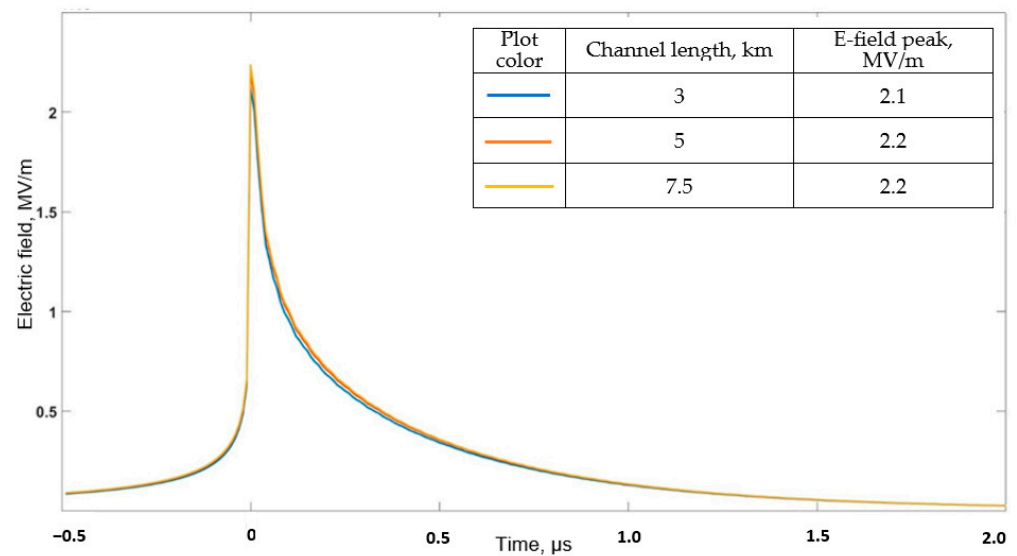
Figure 8. Electric field waveforms at a point located 250 m above ground as the leader passes through it, computed for maximum leader channel lengths of 3 km, 5 km, and 7.5 km. The return-stroke peak current is I_p = 12 kA and the leader speed is 10^7 m/s. Full time scale is 2.5 \mu\text{s} .
