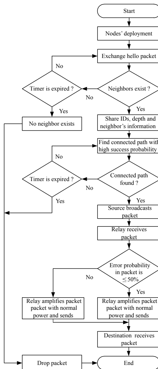
Figure 3. Flow chart of RAR and RACAA.
