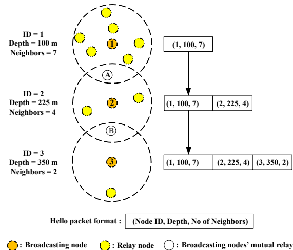
Figure 2. Strategy for sharing ID, depth and neighbors information among one-and-multi-hop neighbor sensor nodes.
