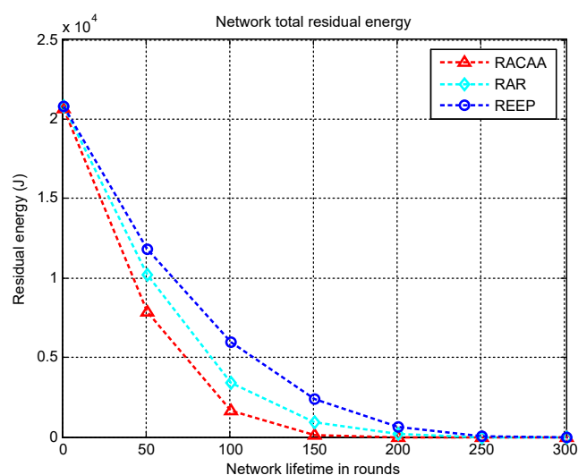
Figure 5. Total residual energy.
