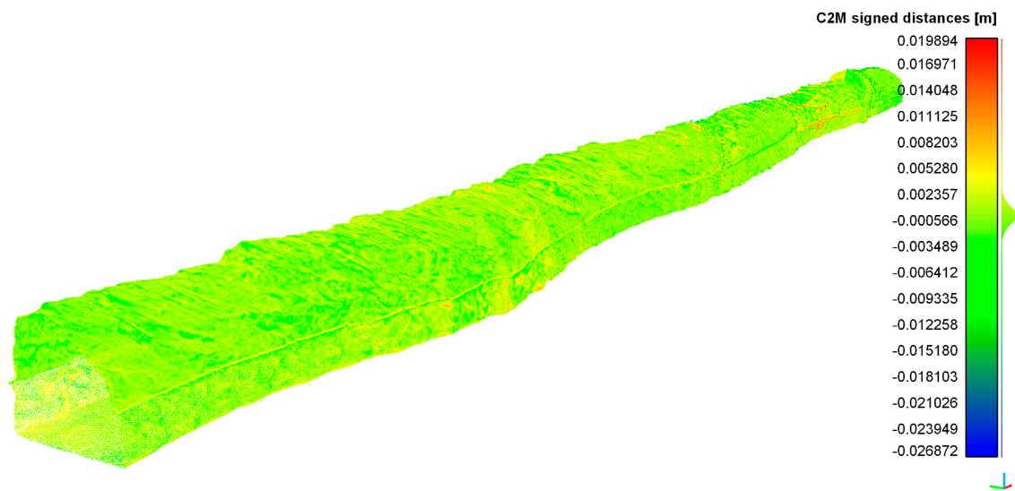
Figure S1: Difference plot between the milling mesh and the coated SfM point cloud defining the digital twin of the Bjørndal 1 model. Note the different colour scale compared to Figure 4 and Figure S2.
