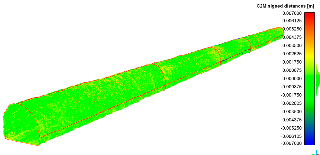
Figure S2: Difference plot between the milling mesh and the coated SfM point cloud defining the digital twin of the Grøndal model. Note the different colour scale compared to Figure 4 and Figure S1.
