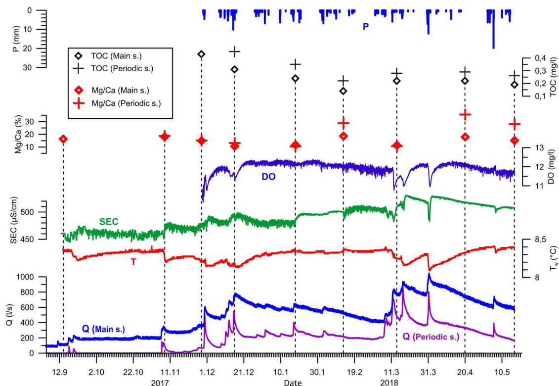
Figure 3. Discharge ( Q ), total organic carbon content (TOC), Mg/Ca molar ratio, and precipitation ( P ) data for both Kravica springs; temperature ( T ), specific electrical conductivity (SEC) and dissolved oxygen (DO) data monitored in the main spring.
