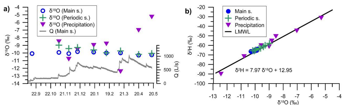
Figure 9. Stable isotope composition of the springs water and local precipitation: (a) Changes of \delta^{18}\text{O} in time and hydrograph of the main spring ( Q ); (b) Composition of \delta^2\text{H} and \delta^{18}\text{O} in all samples, and the local meteoric water line (LMWL) resulting from the bulk precipitation compositions.
