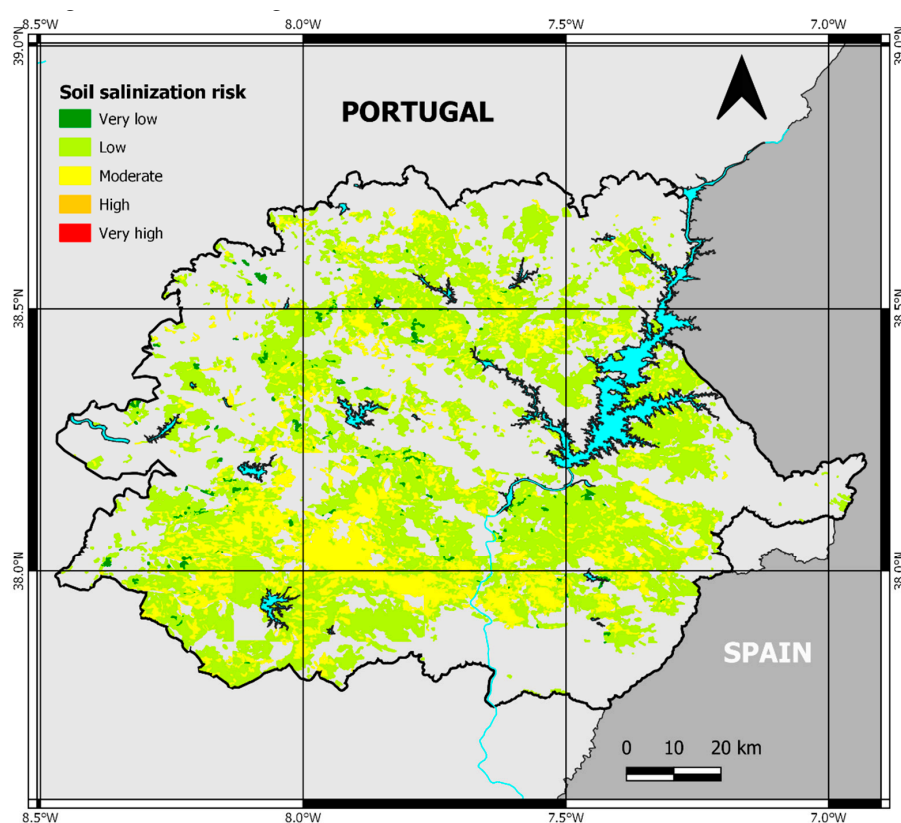
Figure 7. Salinization risk of the potentially irrigated area in the Inland Alentejo region based on the Salinization Risk index (RSA). Very Low risk: RSA < 7; Low risk: 7 ≤ RSA < 10; Moderate risk: 11 ≤ RSA < 14; High risk: 15 ≤ RSA < 18; Very-High risk: RSA > 18.
