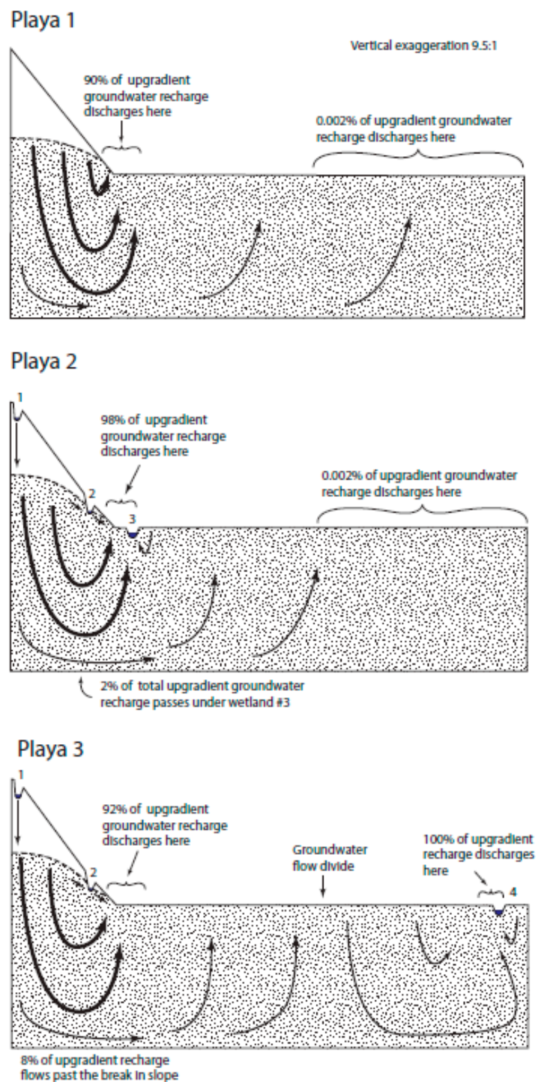
Figure 3. Simulated flow through the Playa landscapes.
