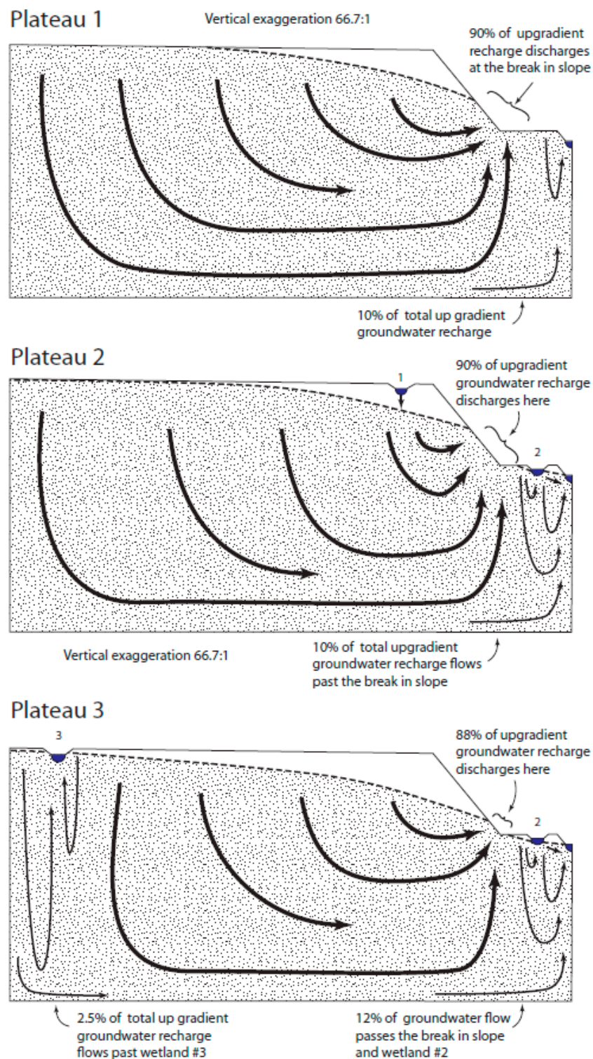
Figure 4. Simulated flow through the Plateau landscapes.
