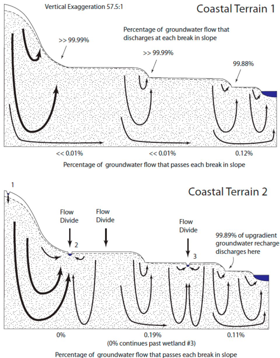
Figure 7. Simulated flow through the Coastal Terrain landscapes.
