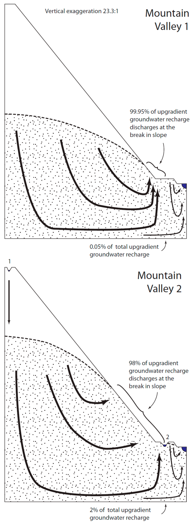
Figure 5. Simulated flow through the Mountain Valley landscapes.
