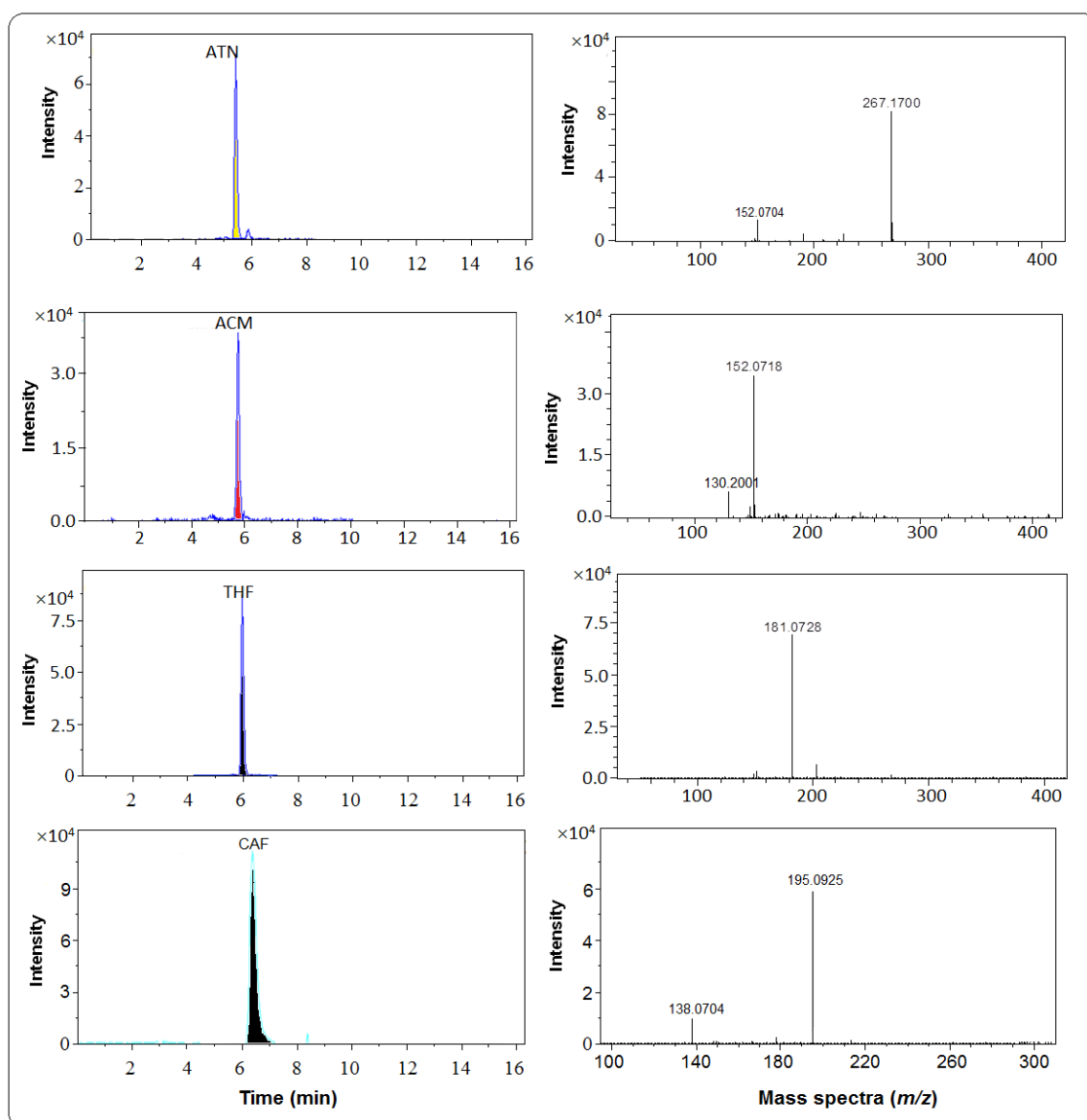
Figure S2. LC chromatograms and mass spectra of some detected pharmaceuticals in STP influent.
