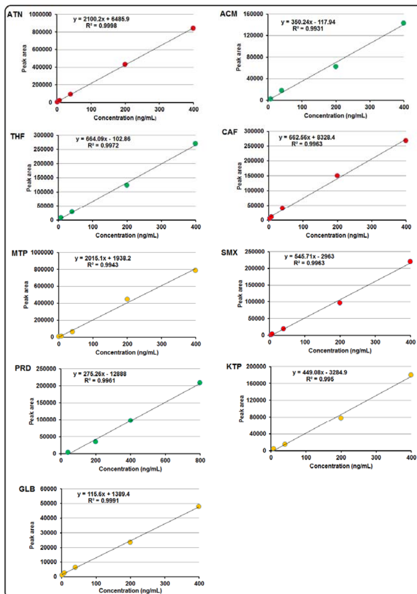
Figure S1. Calibration curve graphs for all studied pharmaceuticals.
