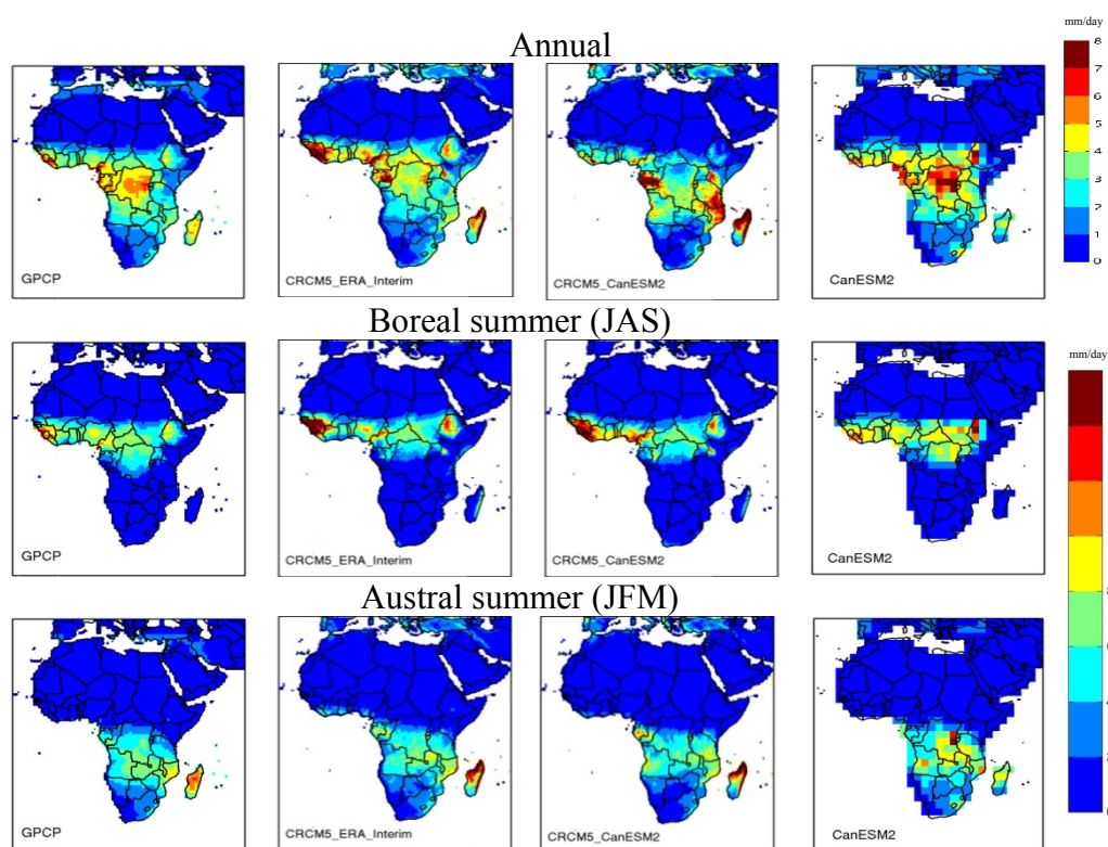
Figure 5. Annual (top row), boreal (middle row) and austral (bottom row) summer mean (1997–2008) precipitation for GPCP (extreme left), CRCM5 driven by ERA-Interim (middle left), CRCM5 driven by CanESM2 (middle right) and CanESM2 (extreme right), for the 1997–2008 period.
