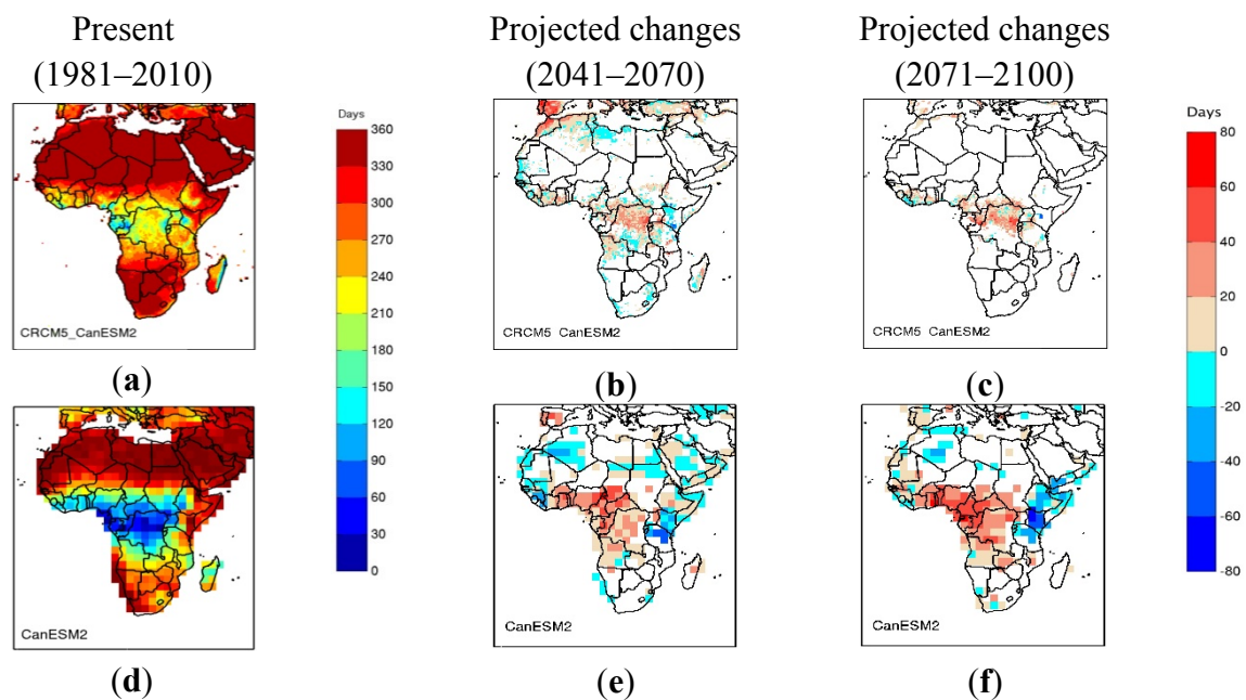
Figure 6. Annual mean number of dry days as simulated by CRCM5 driven by CanESM2 (a–c) and CanESM2 (d–f) for the present (1981–2010) (a,d) and the corresponding projected changes for the 2041–2070 (b,e) and the 2071–2100 (c,f) periods for RCP 4.5 scenario for 2 mm threshold. Grid cells where projected changes are not statistically significant at 95% confidence level are shown in white.
