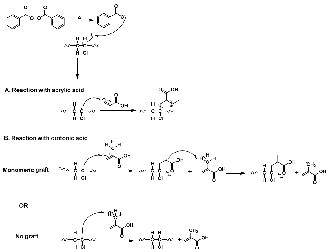
Scheme S1. Schematic reaction mechanism for the grafting of acrylic acid or crotonic acid to the main chain of PVC.
