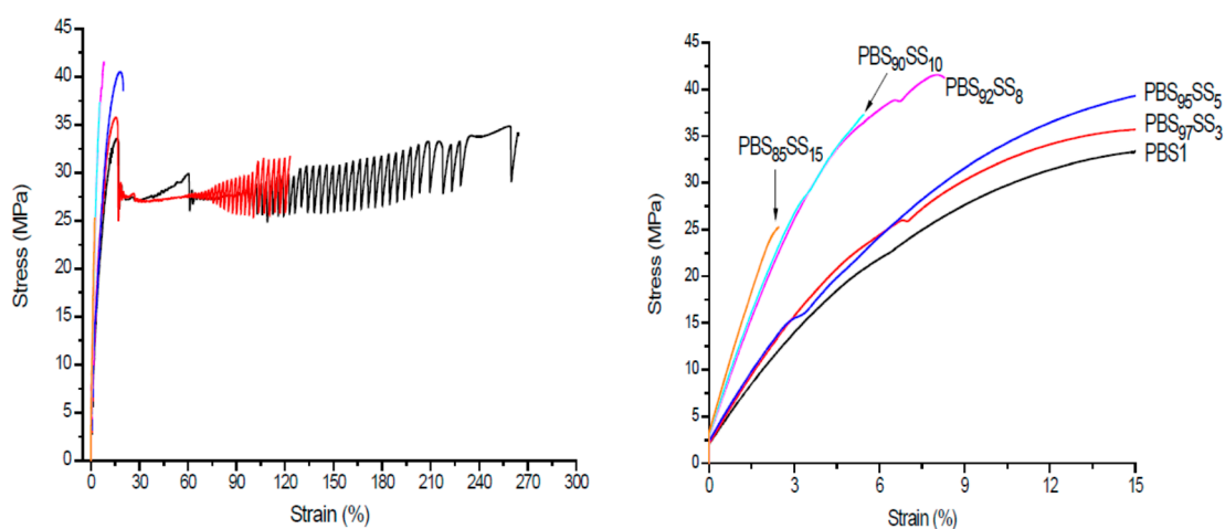
Figure S4. Stress-strain curves of \text{PBS}_x\text{SS}_y copolyesters ( left ). Expanded view of the elastic deformation region ( right ).
