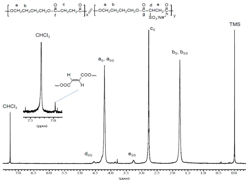
Figure S2. ^1\text{H} NMR spectrum of PBS 85 SS 15 copolyester after heating at 210 °C for 30 min.
