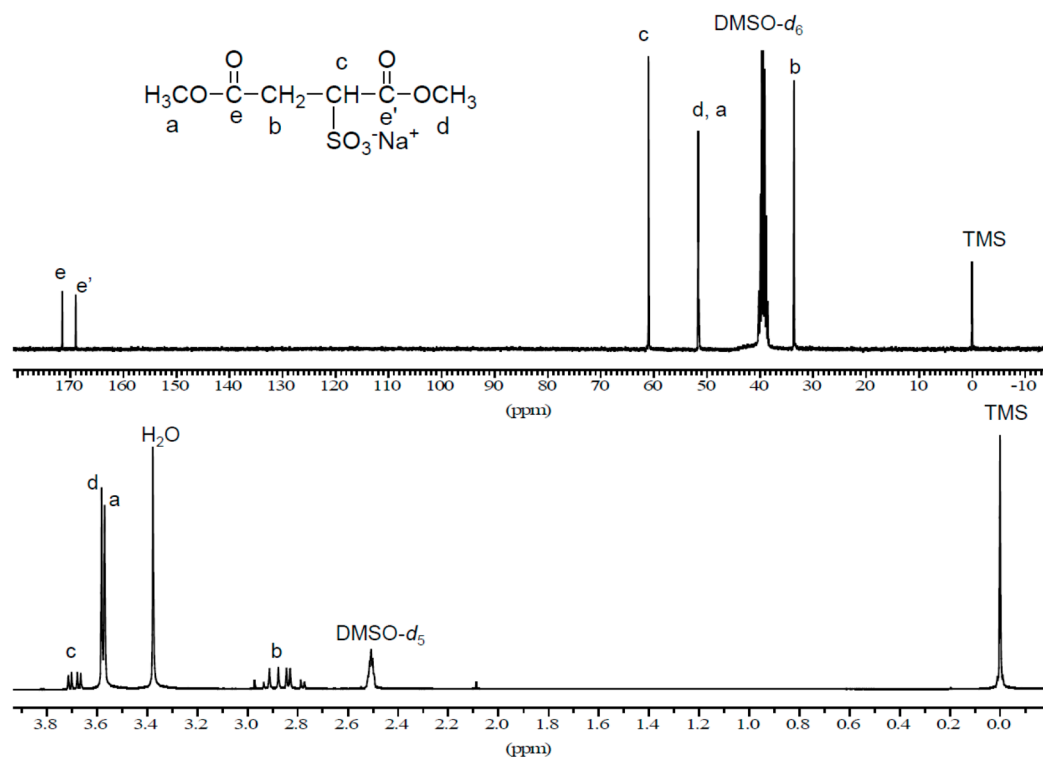
Figure S1. ^1\text{H} NMR (bottom) and ^{13}\text{C} NMR (top) spectra of SDMS.
