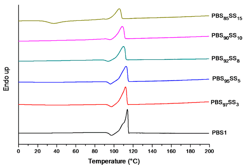
Figure S3. DSC thermograms (second heating) of \text{PBS}_x\text{SS}_y copolyesters.
