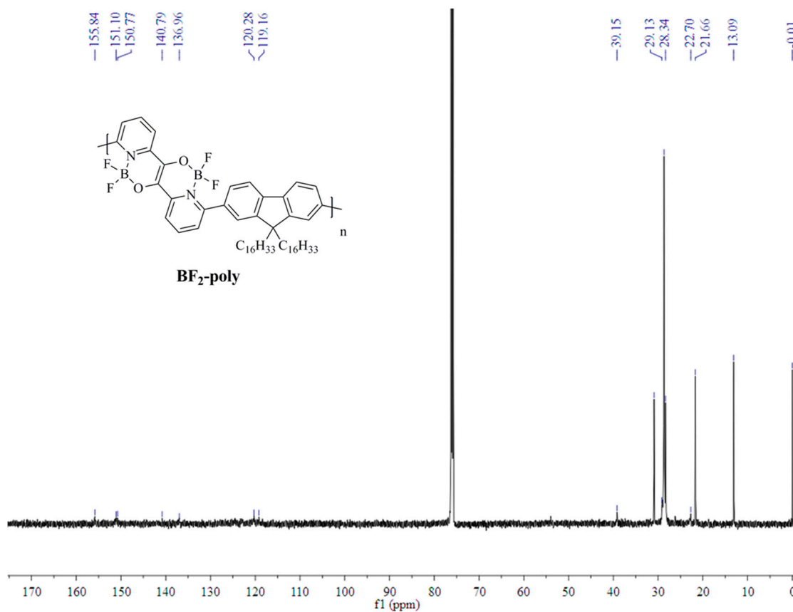
Figure S8. 13 C NMR spectrum of BF 2 -poly.
