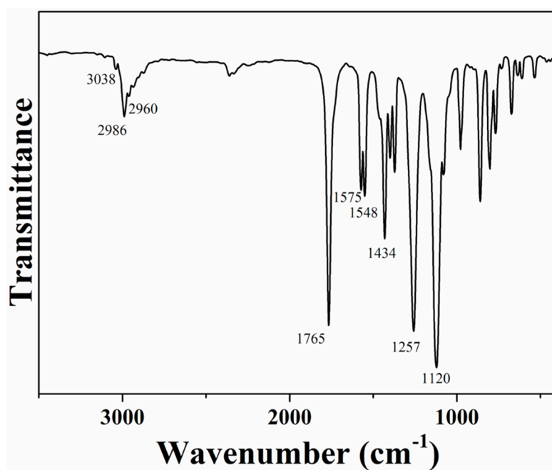
Figure S1. FT-IR spectrum of Monomer 5.
