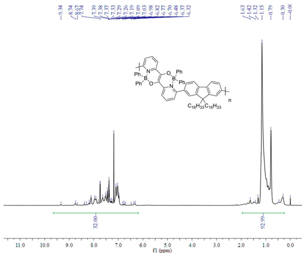
Figure S7. 1 H NMR spectrum of BPh 2 -poly.
