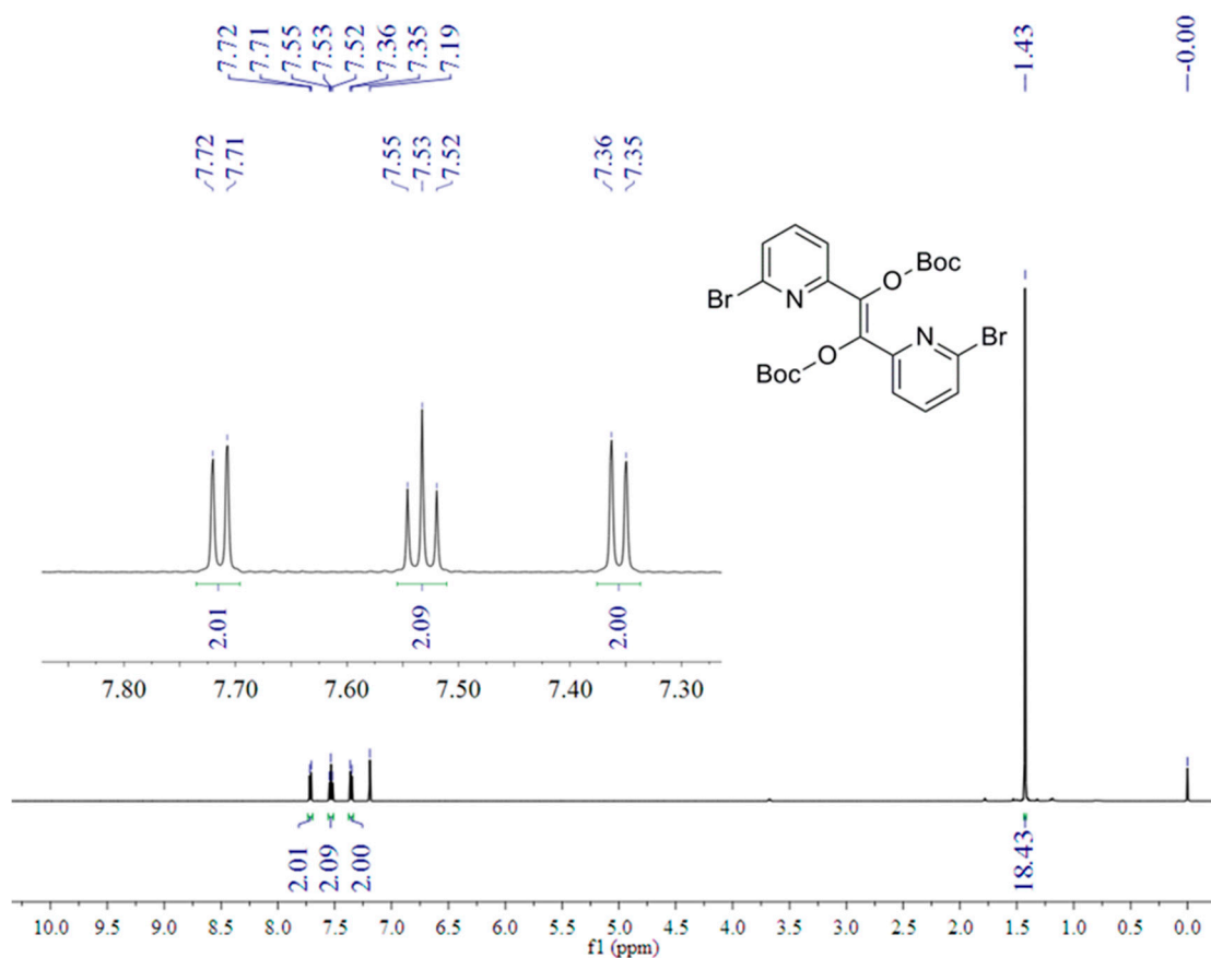
Figure S2. ^1\text{H} NMR spectrum of Monomer 5.
