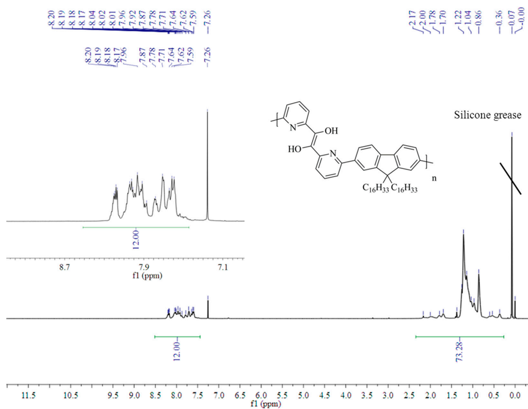
Figure S5. 1 H NMR spectrum of poly-1.
