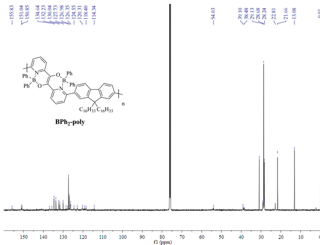
Figure S9. 13 C NMR spectrum of BPh 2 -poly .
