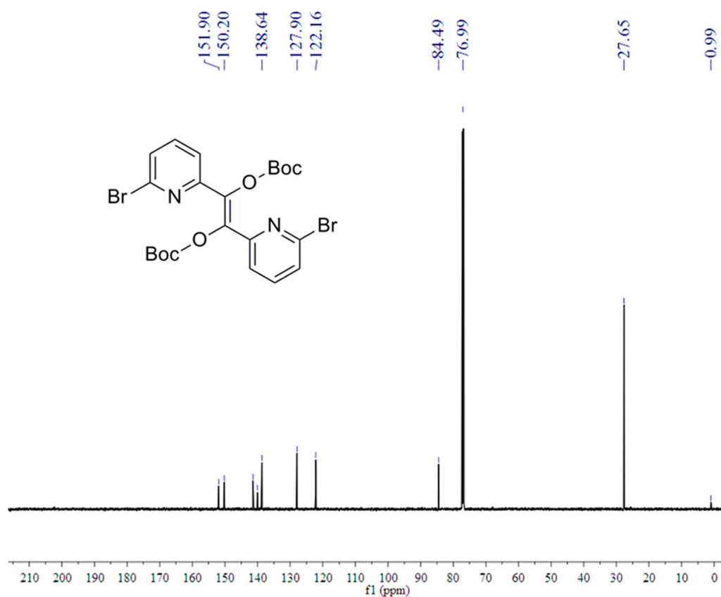
Figure S3. 13 C NMR spectrum of Monomer 5.
