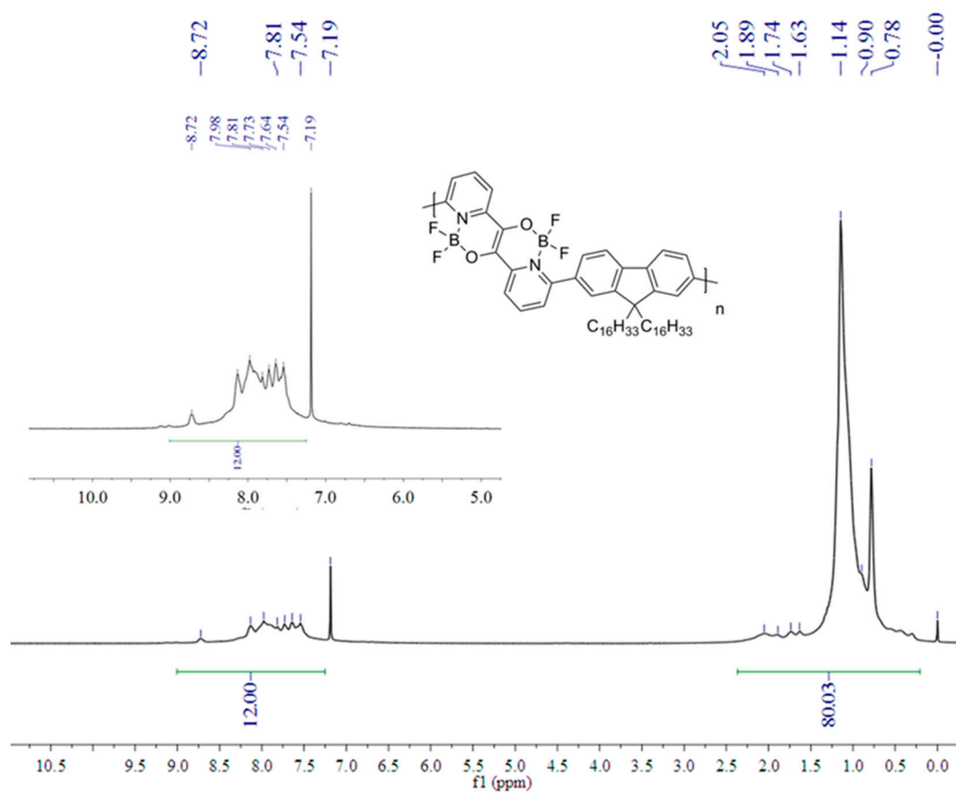
Figure S6. 1 H NMR spectrum of BF 2 -poly.
