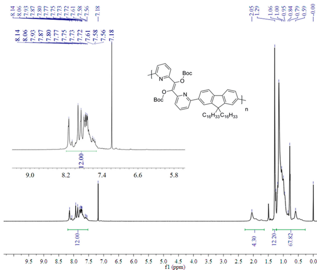
Figure S4. 1 H NMR spectrum of Boc-poly.
