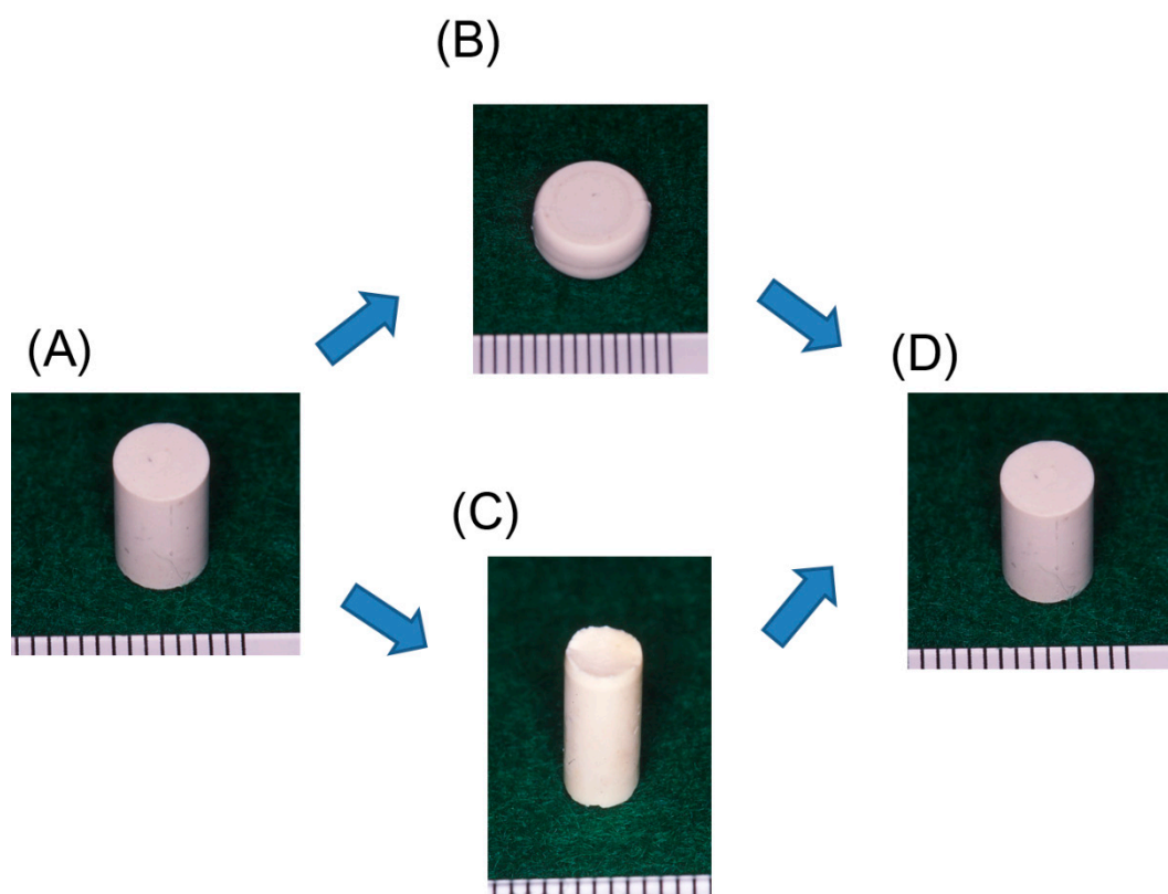
Figure S2. Photograph of the cylindrical test specimen: (A) original shape (diameter-6.0 mm); (B) deformed shape (30% compressed); (C) deformed shape (diameter-4.6 mm); (D) recovery shape.
