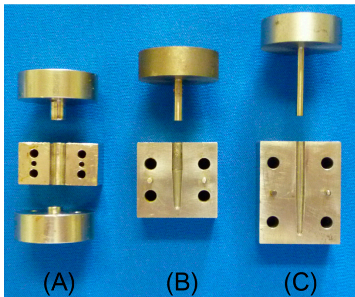
Figure S1. Photograph of the split-type metal mold (A) for preparing the cylindrical test specimen; (B) for preparing the trial point; (C) for deformation of the trial point.
