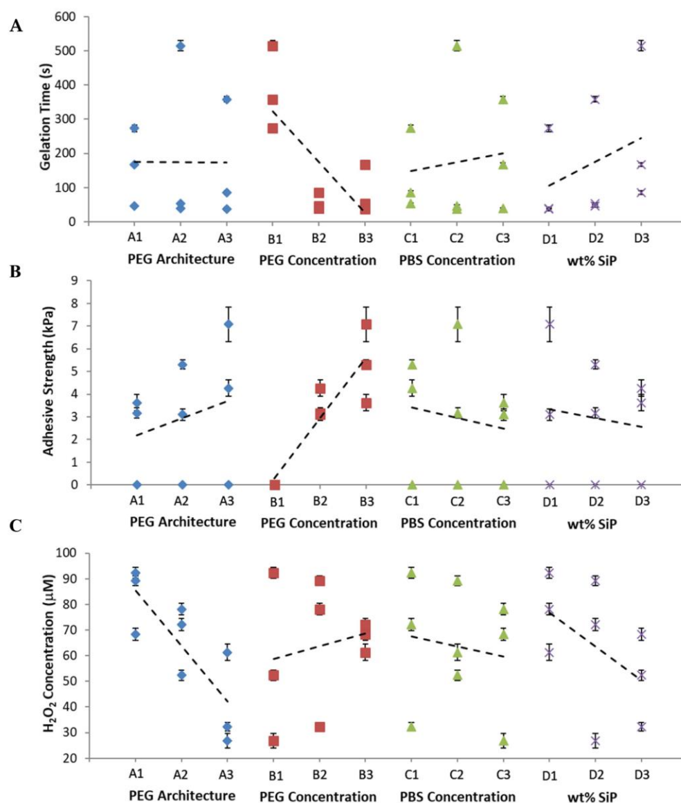
Figure 1. Average gelation time (A), adhesive strength (B), and \text{H}_2\text{O}_2 concentration (C), based on the 9 adhesive formulations from Table 2. Values are plotted as means and standard deviations of experimental values for the corresponding factor levels. The dashed lines are linear trend lines.
