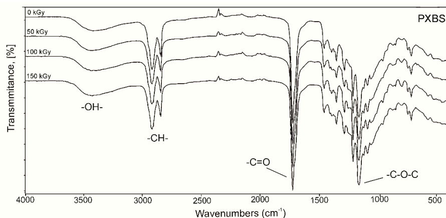
Figure S3. FTIR spectra of poly(xylitol sebacate-co-butylene sebacate) (PXBS) before and after irradiation.
