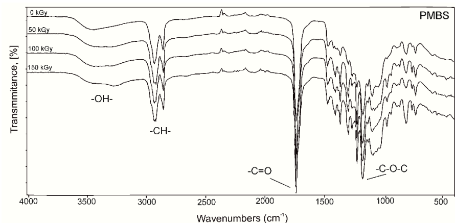
Figure S5. FTIR spectra of poly(mannitol sebacate-co-butylene sebacate) (PMBS) before and after irradiation.
