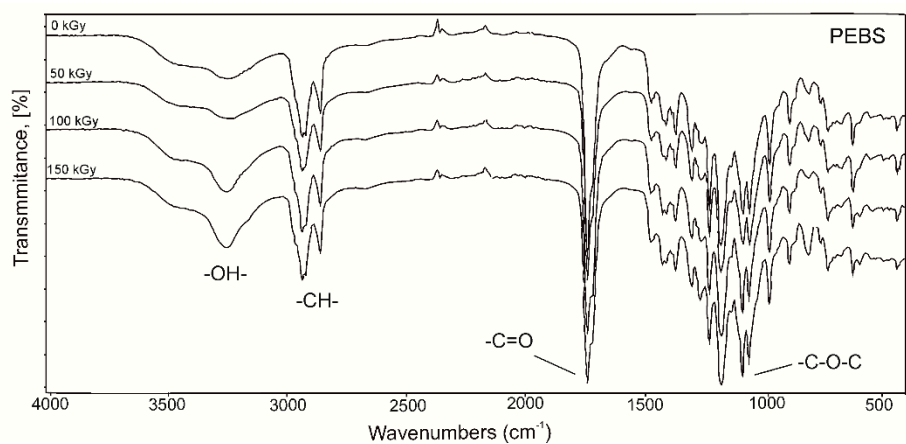
Figure S2. FTIR spectra of poly(erythrytol sebacate-co-butylene sebacate) (PEBS) before and after irradiation.
