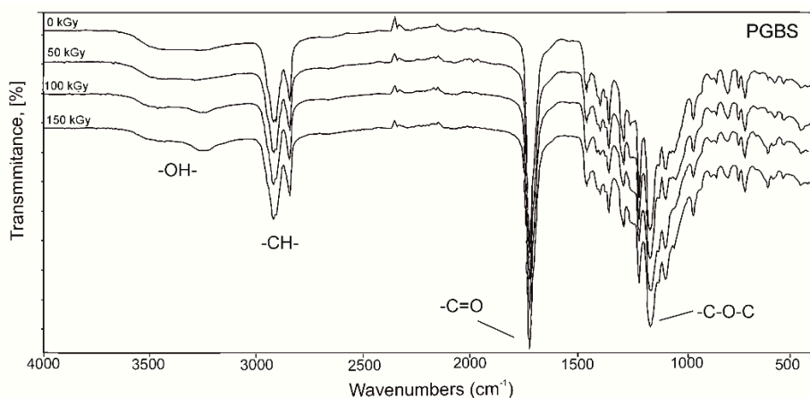
Figure S1. FTIR spectra of poly(glycerol sebacate-co-butylene sebacate) (PGBS) before and after irradiation.
