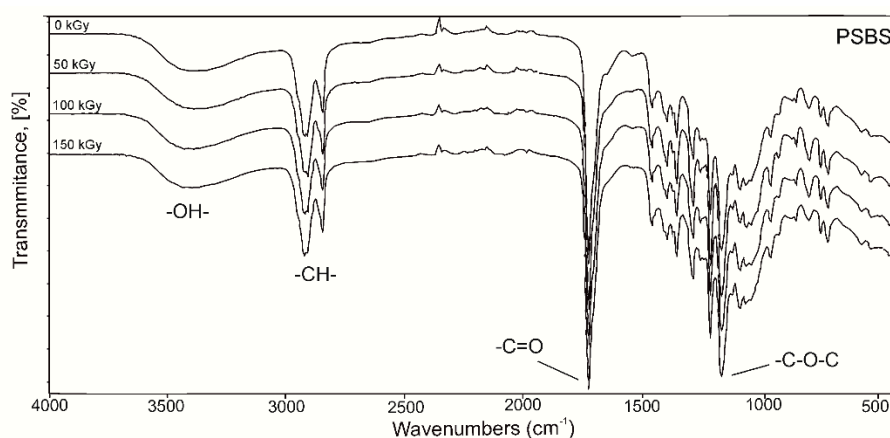
Figure S4. FTIR spectra of poly(sorbitol sebacate-co-butylene sebacate) (PSBS) before and after irradiation.
