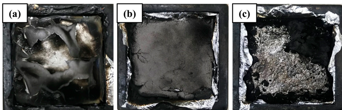
Figure S1. The digital photos of the residual char after cone calorimetry test of (a) PU–RH, (b) PU–RH/ATH, and (c) PU–RH/OP.
