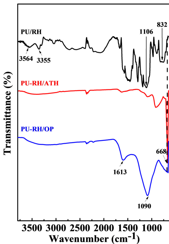
Figure S2. FTIR spectra of PU–RH and PU–RH/FR residues after cone calorimetry test.
