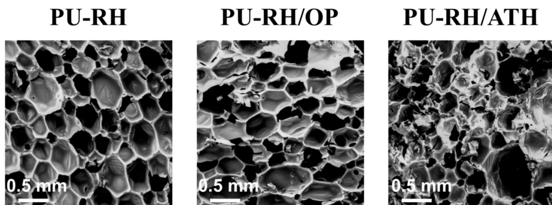
Figure S3. SEM micrographs of PU-RH and PU-RH/FR residues after cone calorimetry test.
